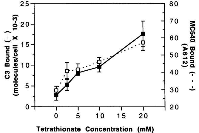
Figure 3. Membrane phospholipid redistribution and complement activation on normal erythrocytes after treatment with sodium tetrathionate. Erythrocytes were treated with 0–20 mM sodium tetrathionate for 1 h at 37°C. MC540 binding that correlates with PE and PS exposure was measured fluorimetrically (open squares, dotted lines). Treated erythrocytes were incubated with MgEGTA-treated autologous serum, washed, lysed, and deposited C3 was measured by a competitive ELISA (closed squares, solid lines). Means \pm SEM are shown for four experiments.
