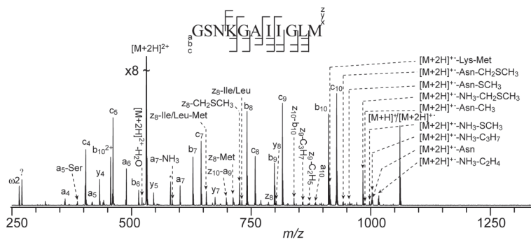
Figure 2. ECD spectrum of amyloid β peptide (25-35). Peak labeling follows the same convention as in Figure 1. The cleavage pattern is shown as the inset. (Reprinted with permission from reference [47].)
