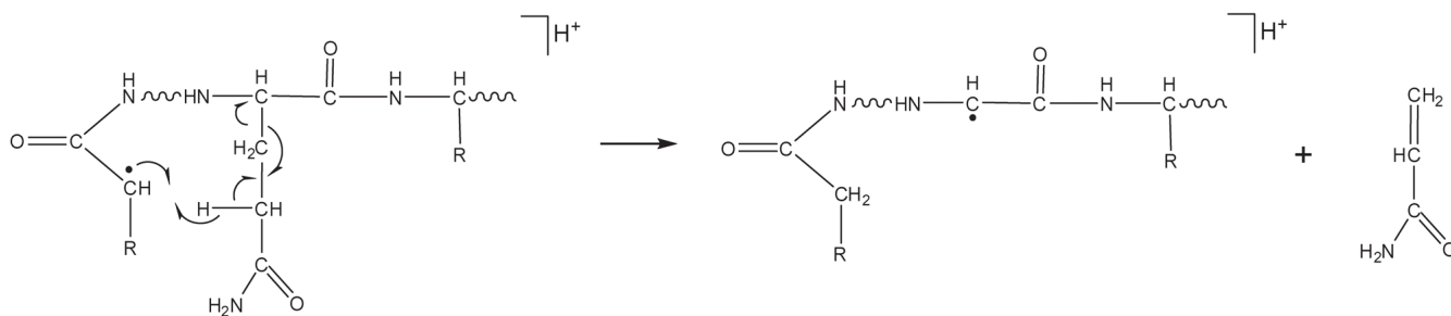
Scheme 1. Entire side chain loss from z• ions via gamma hydrogen abstraction.
