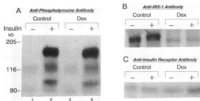
Figure 1. Insulin-stimulated tyrosine phosphorylation in intact muscle from dexamethasone-treated rats. Rats were anesthetized and the abdominal wall was incised to expose the viscera. 1 ml of normal saline (lanes 1 and 3) or 10^{-5} M insulin (lanes 2 and 4) was infused into portal vein as a bolus injection, and 90 s later, muscles were excised and homogenized in extraction buffer B at 4^\circ\text{C} as described in Methods. After centrifugation, aliquots with same amount of protein were resolved on 6% SDS-polyacrylamide gel, transferred to nitrocellulose, and detected with antiphosphotyrosine antibody (A), anti-IRS-1 antibody (B), or antiinsulin receptor antibody (C), and [ ^{125}\text{I} ]protein A, and subjected to autoradiography. Dex, dexamethasone.
