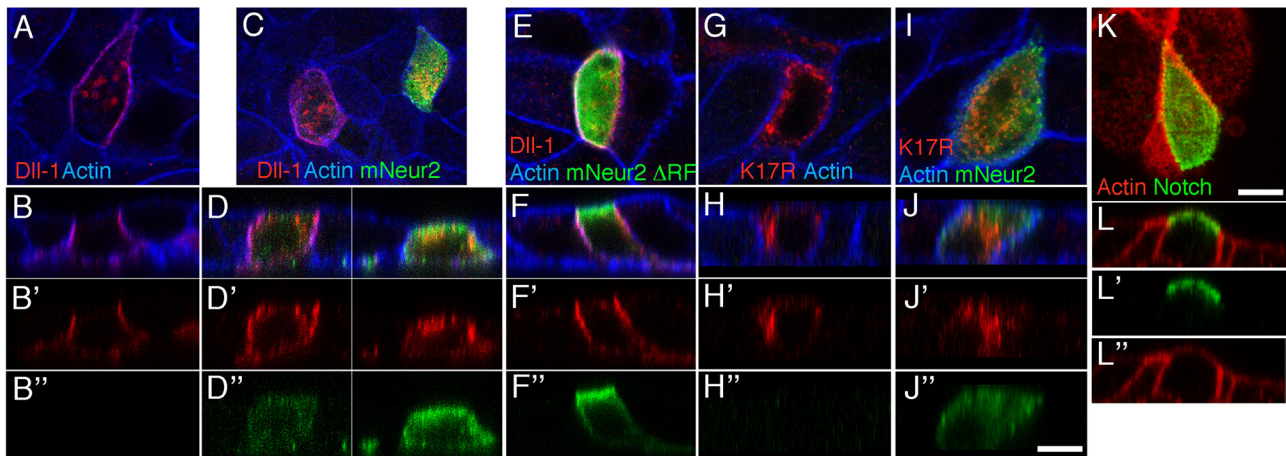
Figure 4. Apical-basal localization of Notch and Dl in polarized MDCK cells. Distribution of a VSV-G-tagged version of wild-type murine Dll-1 (A–F''), red) or K17R Dll11 a mutant version of Dll1 (G–J'') in polarized MDCK cells (phalloidin in blue) in the absence of mNeur2 (A–B'') or the presence of mNeur2 (C–D'', I–J'') or mNeur2-ΔRF (E–F'') (in C–J''); mNeur2 was detected using the HA tag in green). B–B'', D–D'', F–F'', H–H'', and J–J'' show confocal Z-sections of images shown in A, C, E, G, and I, respectively. (K–L'') Distribution of murine Notch1 (green) in polarized MDCK cells (phalloidin in red). Apical is up. Bar, 10 μm (A–H'', J–J'').
