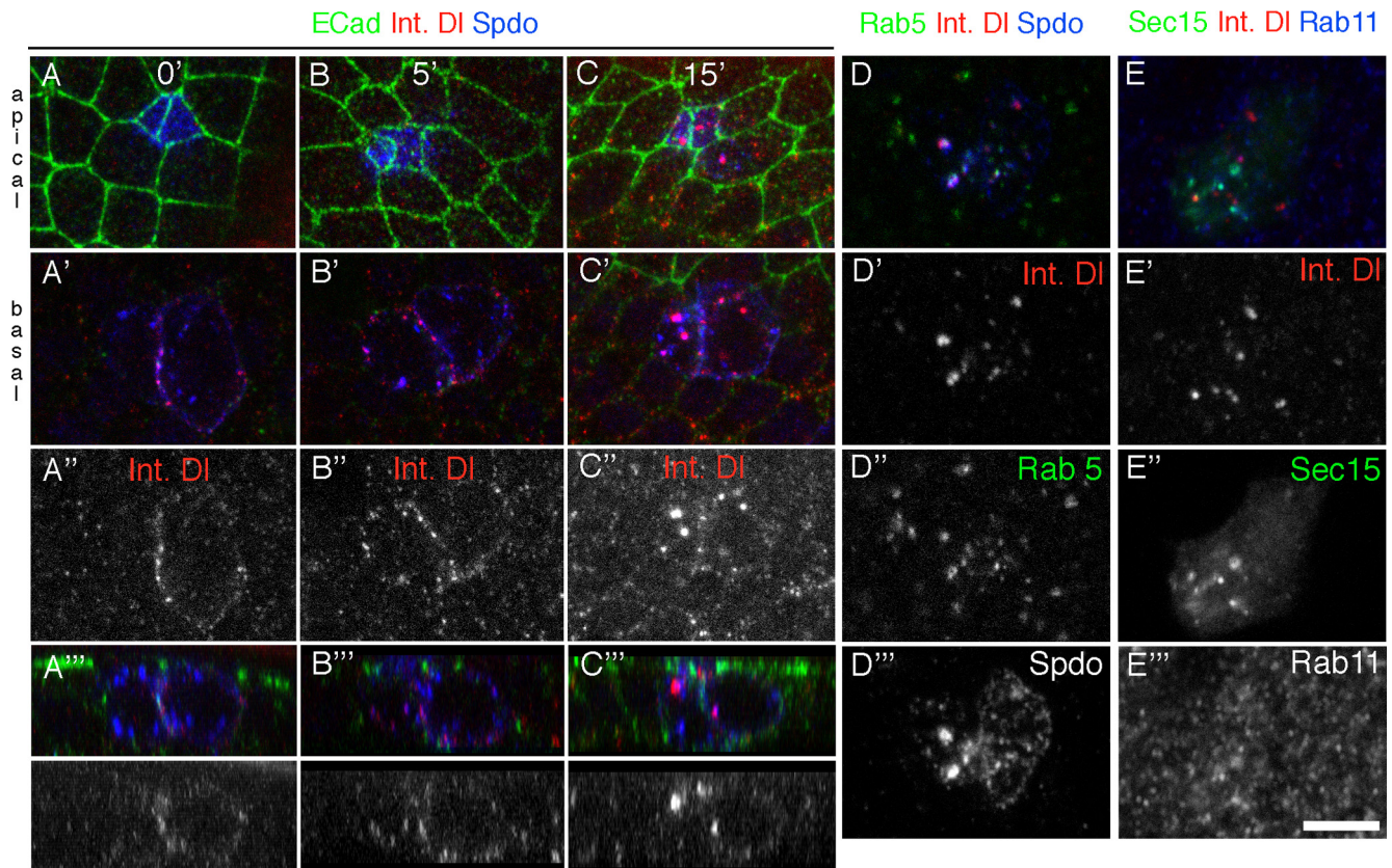
Figure 3. D \Delta is internalized from the basolateral membrane in the pupal notum. (A–C'') Pulse-chase labeling experiments to monitor D \Delta internalization in living pupae. D \Delta internalization (red in A–C'') and separate channel in A'–C'') at the pIIa/pIIb cell stage was examined at three time points (0, 5, and 15 min). A–C show confocal sections at the apical cortex taken at the level of the adherens junctions labeled with E-Cad (green), whereas panels A'–C' show confocal sections taken at the level of the nuclei (basolateral cortex). Sensory organ cells were identified using Spdo (blue in A–C, A'–C'', and D). At 0 min, D \Delta was detected at the basolateral plasma membrane of the pIIa cell as well as at the pIIa/pIIb interface, below E-Cad (green). After 5 min of internalization, clustered D \Delta still present at the plasma membrane and/or small endocytic vesicles containing D \Delta were detected in both pIIa and pIIb cells. At 15 min, D \Delta was predominantly detected in vesicular compartments within the pIIa and pIIb cells. Most of these vesicles were located in vicinity to E-Cad-positive junctions of the pIIb cell. A'–C' show confocal sections along the z-axis of images A–C', respectively. D–E'', distribution of D \Delta 15 min after internalization (D, D', E, E'; red in D, E) relative to Rab5-GFP (D, D'; green in D), Sec15-GFP (E, E'; green in E) and Rab11 (E, E''; blue in E). Sensory organ cells were identified using Spdo (blue in A–C', A'–C'', C'–D and E). Anterior is left. Bars, 10 \mu m.
