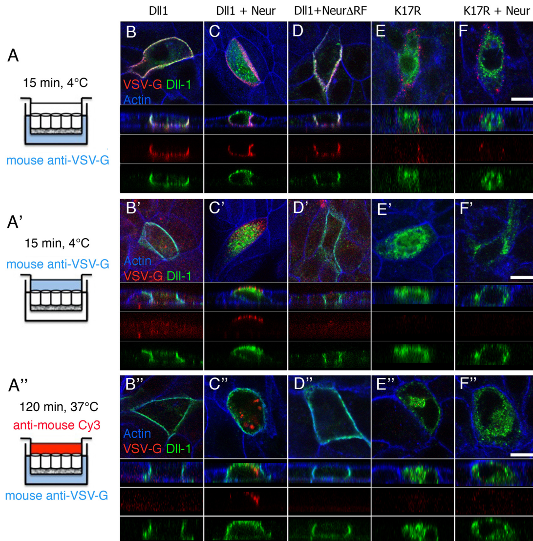
Figure 5. Neur promotes basal to apical transcytosis of DI in MDCK cells. (A–A'') Schematic representation of the cell surface accessibility assay (A and A') and transcytosis assay (A''). (B–F'') Polarized MDCK cells were transfected with VSV-G–tagged mouse Dll-1 (B–D'') or K17R Dll1 (E–F'') alone or together with wild type mNeur2 (C–C'', F–F''), or mNeur2- \Delta RF (D–D''). They were then incubated with anti-VSV-G antibodies in the basal (A, B–F) or apical compartment (A', B'–F') at 4°C for 15 min. Alternatively, polarized MDCK cells were incubated with anti-VSV-G and anti-mouse Cy3 in the basal and apical compartment respectively for 120 min at 37°C (A'', B''–F''). Dll-1 was detected using rabbit anti-Dll-1 (green; phalloidin in blue). Orthogonal confocal sections taken along the z-axis are shown below images B–F''. The faint diffuse red staining seen in B'', D'', E'', and F'' corresponds to background (laser intensity and detector sensitivity of the confocal were increased compared with C''). Bar, 10 \mu m (B–F') and 5 \mu m (B'–F'').
