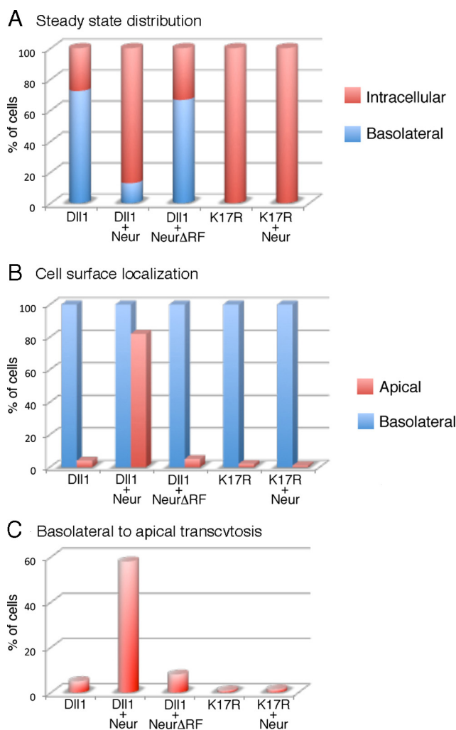
Figure 6. Quantitation of Dll-1 localization and transcytosis in polarized MDCK cells. (A) Steady-state distributions of Dll-1 ( n = 48 ), Dll-1 + mNeur2 ( n = 47 ), Dll-1+mNeur2- \Delta RF ( n = 47 ), K17R Dll-1 (K17R; n = 45 ), and K17R Dll1 + mNeur2 ( n = 50 ). In this semiquantitative analysis of confocal images, basolateral staining refers to cells in which Dll1 was predominantly observed at the basolateral membrane (see Figure 4, A, B and E, F). In cells where Dll1 predominantly localized in intracellular compartment (see Figure 4, C, D and G–J’), staining was classified as intracellular. (B) Quantitation of apical and basolateral cell surface immunostaining of Dll-1 ( n = 49 and n = 46 , respectively), Dll-1 + mNeur2 ( n = 68 and n = 60 , respectively), Dll-1 + mNeur2- \Delta RF ( n = 54 and n = 48 , respectively), K17R Dll1 ( n = 49 and n = 56 , respectively), and K17R Dll1 + mNeur2 ( n = 45 and n = 58 , respectively) illustrated in Figure 5, B–F and B–F’. Numbers into brackets refer to the number of cells analyzed for apical and basolateral cell surface staining, respectively. Apical versus basolateral cell surface staining was done on separate transwell filters. In this quantitation the occurrence of the immunostaining (binary: yes or no) at the apical or basolateral membrane was assessed. All transfected cells exhibited a basolateral staining, including cells transfected with K17R Dll1 mutant that showed low plasma membrane staining. This apparent discrepancy is likely due to the fact that the anti-VSVG antibody is more sensitive than anti-Dll1. By contrast, apical staining was almost exclusively detected upon coexpression of mNeur2 and Dll-1 (80% of the cells expressing Dll1 showed a VSG-G staining at the apical surface). (C) Quantitation of basal to apical transcytosis of Dll-1 ( n = 49 ), Dll-1 + mNeur2 ( n = 90 ), Dll-1 + mNeur2- \Delta RF ( n = 54 ), K17R Dll1 ( n = 56 ), and K17R Dll1 + mNeur2 ( n = 58 ) as shown in Figure 5, A’–F’’. In all cases, quantitation was performed on results obtained from at least three independent experiments. Experiments performed in parallel indicated that mNeur2 and Dll-1 constructs are typically coexpressed in 90% of transfected cells.
