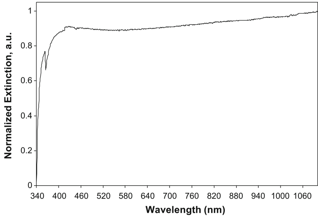
Fig. 8. Extinction spectrum of PLGA-Ag nanocages.
