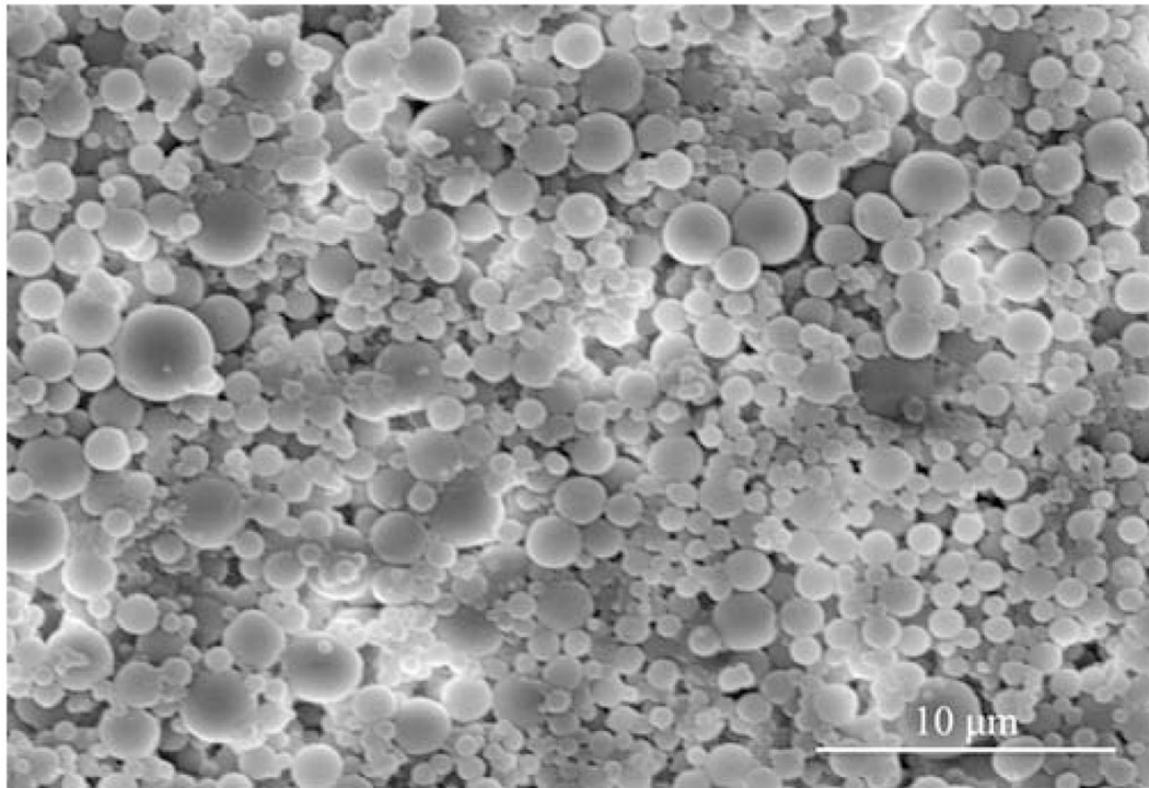
Fig. 3. SEM image of PLGA W/O/O submicron particles formed using 120 W sonication for the creation of the second emulsion.
