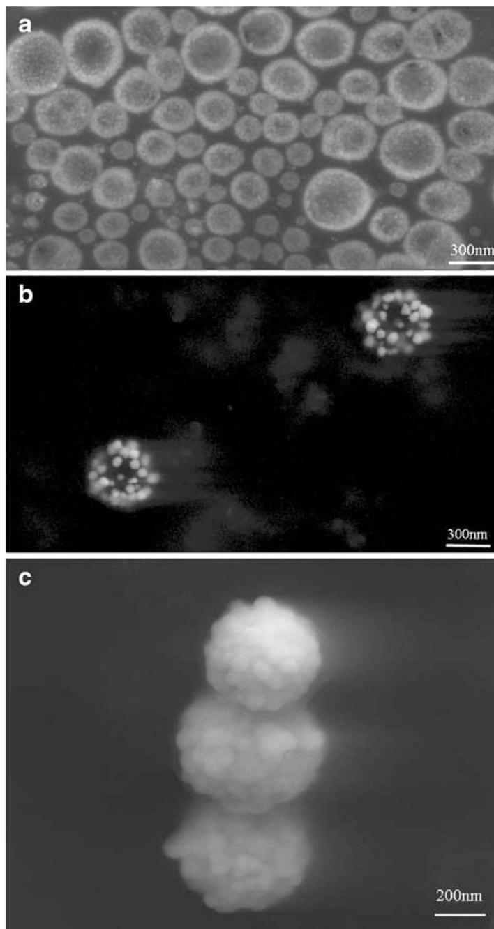
Fig. 5. PLGA-Ag nanocages at various stages of silver reduction, a silver seeds coating PLGA following photoreduction, b intermediate step in the ascorbic acid reduction where larger seeds on PLGA are present, c final porous cage configuration of silver on PLGA at the completion of ascorbic acid silver reduction.
