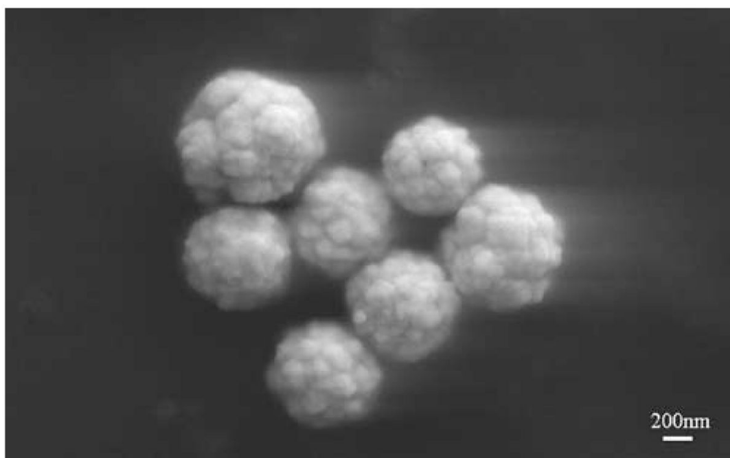
Fig. 6. SEM image of the W/O/O particles with encapsulated rhodamine and a silver cage on the exterior of the particle.
