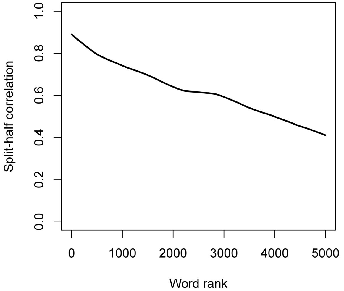
Figure 1. Loess-smoothed plot of split-half reliability estimate as a function of word rank (ranked by frequency of occurrence in the corpus).
