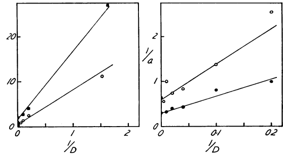
FIG. 4. PLOT OF THE RECIPROCAL OF THE AMOUNT OF IRON ABSORBED ( 1/a ) VS THE RECIPROCAL OF THE AMOUNT OF IRON IN THE DOSE ( 1/D ). Note that there is a difference in the coordinates in each figure; the figure on the right includes an expansion of the origin of the figure on the left for the normal mice, group N. ■ = Group Fe, ○ = group N, and ● = group D.
