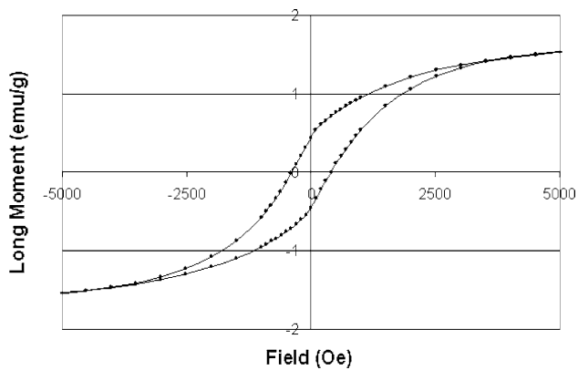
Fig. 2 Magnetization curve
