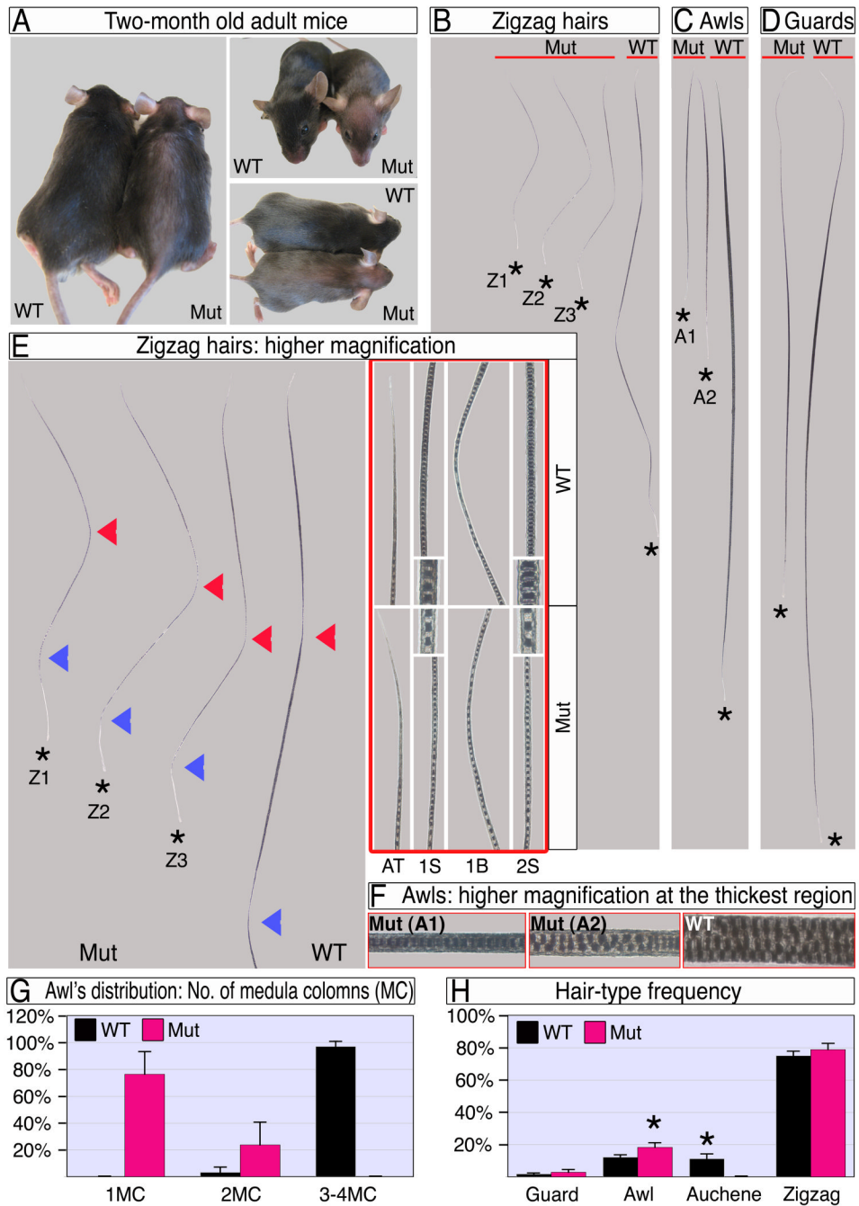
Figure 2. Ablation of \beta -catenin in the DP results in dramatic hair shortening and thinning (A) Adult wild type and mutant mice. Note the epidermis is visible through the thin mutant hair coat. (B–D) Zigzag, awl and guard hair-types after the first hair cycle. The apical tips of all hairs are aligned next to the red line and hair-clubs are marked by stars. Mutant hairs within a hair-type population are classified into sub-types based on their different length and/or thickness. Z1–Z3 in B represent a first segment 50% or less, between 50–100%, and similar in length to wild type respectively. A1–A2 in C represent 1 or 2 columns of medulla cells respectively. (E) Mutant zigzag hairs and the apical portion of a wild type zigzag are shown at left. The first and second bends from the apical tip are marked by red and blue arrowheads, respectively. At right, framed with red line, higher magnifications of the apical tip (AT), mid-
