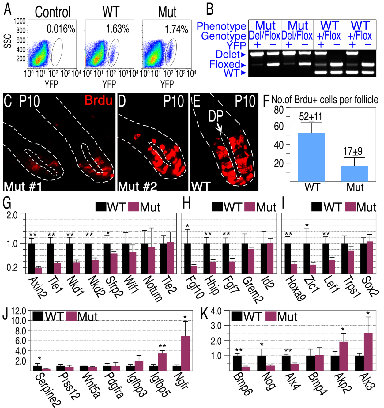
Figure 3. Deletion of \beta -catenin in the DP results in reduced proliferation rates of matrix cells and alterations of gene expression in the DP
