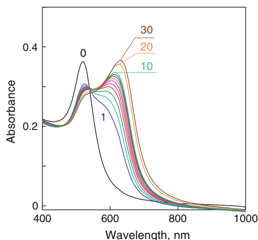
Fig. 1 Time-dependent absorption spectra of NPs–Gm mixture (1:1 v/v). The final concentration of NPs and Gm are 0.15 mM and 0.05 μg mL -1 , respectively. The numbers near curves designate the time after mixing (seconds), the curve 0 is the initial spectrum without Gm
