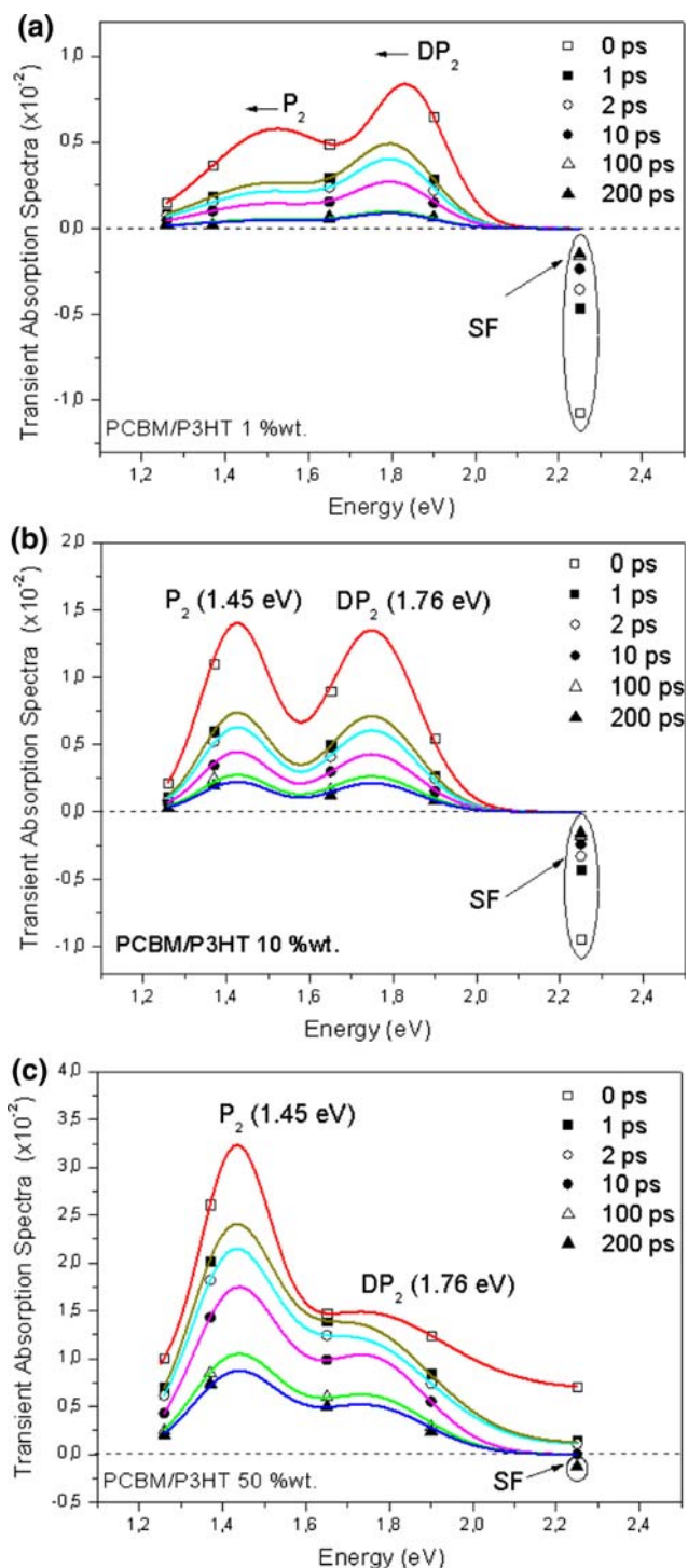
Fig. 2 Transient absorption spectra for P3HT/PCBM blend materials with 1 (a), 10 (b), and 50 wt% (c) PCBM concentration. The spectra measured at 0 ps (open squares), 1 ps (full squares), 2 ps (open circles), 10 ps (full circles), 100 ps (open triangles), and 200 ps (full triangles), respectively, following the pulse excitation at 3.8 eV. The P_2 , DP_2 , and SF bands are assigned. The color curves represent the fits using a superposition of two Gaussian peaks centered at the reported values of polaron states in the literature [5]
