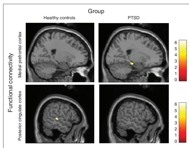
Fig. 1: Functional connectivity with the medial prefrontal cortex and the posterior cingulate cortex seed regions (thresholded at p = 0.001 , uncorrected). The patients with posttraumatic stress disorder (PTSD) showed significant connectivity with the parahippocampal gyrus during the working memory updating task. The control group showed significant connectivity with the superior temporal gyrus during the working memory updating task.
