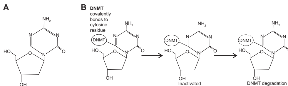
Figure 1 Structure and trapping mechanism of decitabine. A) The chemical structure of decitabine (4-amino-1-(2-deoxy-β-D-erythro-pentofuranosyl)-1,3,5-triazin-2(1H)-one, C_8H_{12}N_4O_5 ). B) The action of the DNMTs is inhibited by decitabine-incorporated DNA. Covalently trapped DNMTs are degraded, leading to depletion of cellular DNMTs.
