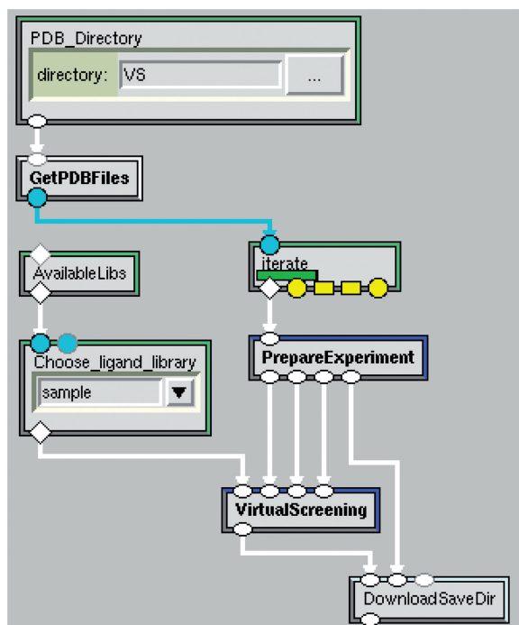
Figure 4. Autodock virtual screening workflow in Vision. A user may specify an input directory, e.g. VS, which contains one or more PDB files, corresponding template GPFs and DPFs. A user may select a ligand library from the list of libraries. After the virtual screening job finishes, the top 500 docking results along with summarized results are automatically downloaded to the user's local machine.
