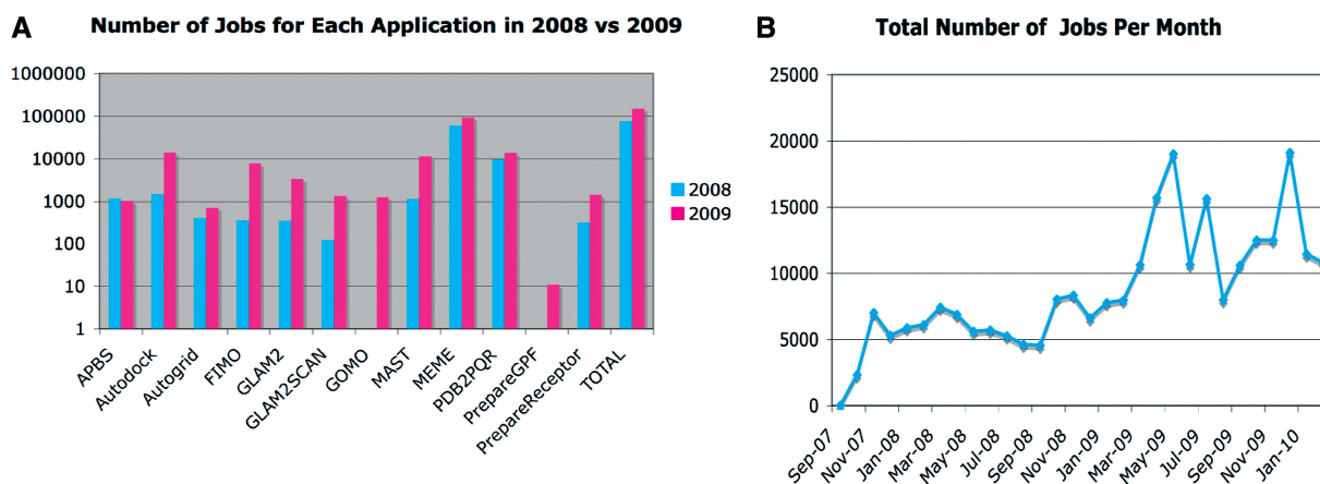
Figure 2. (A) Comparison of numbers of jobs successfully executed in 2008 and 2009 in a semi-log graph. (B) Number of total jobs successfully executed per month.
