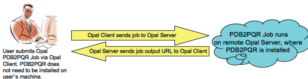
Figure 3. Opal client/server architecture – running a PDB2PQR job as a Web service call.
