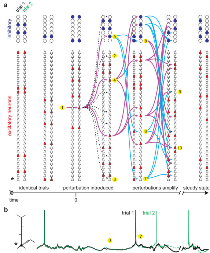
Figure 1. The effect of an extra spike
