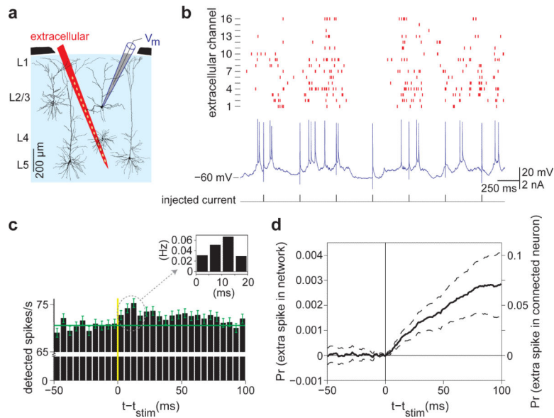
Figure 4. The effect of one extra spike on network activity
