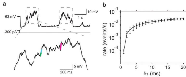
Figure 5. Precisely timed events are rare
