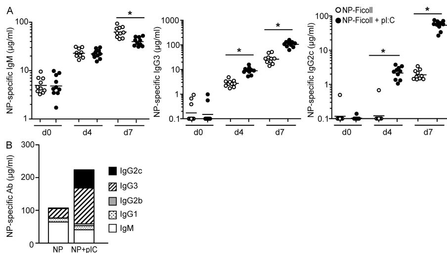
Figure 1. Poly(I:C) enhances the antibody response to a model TI-2 antigen. (A) C57BL/6 mice were immunized with 5 µg NP-Ficoll alone or 5 µg NP-Ficoll + 100 µg poly(I:C) and serum NP-specific IgM, IgG3, and IgG2c antibodies were measured in preimmune (day 0 [d0]), day 4, and day 7 after immunization sera. Symbols represent individual mice, and horizontal bars indicate geometric mean. Data were combined from two independent experiments with five mice per group per experiment. *, P \leq 0.005 . (B) Total serum NP-specific IgG2c, IgG3, IgG2b, IgG1, and IgM were measured 7 d after immunization with NP-Ficoll ± poly(I:C). Data represent geometric means calculated from data combined from two independent experiments, with five mice per group per experiment. Geometric means from NP-specific IgM, IgG3, and IgG2c responses were the same as those represented in A.
