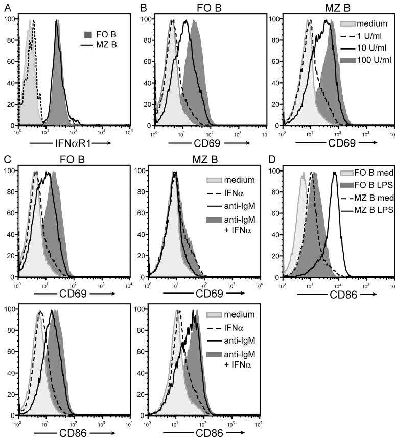
Figure 6. IFN- \alpha induces BCR-stimulated FO B cells to up-regulate CD69 to a greater extent than MZ B cells. (A) Histograms represent flow cytometric analysis of IFN \alpha R1 surface expression on CD21 int CD23 high FO B cells and CD21 high CD23 low MZ B cells isolated from naive wild-type mice. Isotype control antibody staining for both FO (shaded light gray) and MZ (dashed line) B cells is provided. Data are representative from two independent experiments. (B–D) FO and MZ B cells were sorted to \geq 94\% purity from naive C57BL/6 mice and separately incubated with the indicated stimuli in vitro for 6 or 10 h. After stimulation, surface expression of CD69 (6 h) or CD86 (10 h) was subsequently assessed in both B cell populations by flow cytometry and data depicted as histograms. The following stimuli and doses were used: (B) rIFN- \alpha at 1, 10, or 100 U/ml; (C) rIFN- \alpha at 1 U/ml and anti-IgM F(ab') 2 at 10 \mu g/ml; (D) LPS at 10 \mu g/ml. Med, medium. Data are representative from at least two independent experiments.
