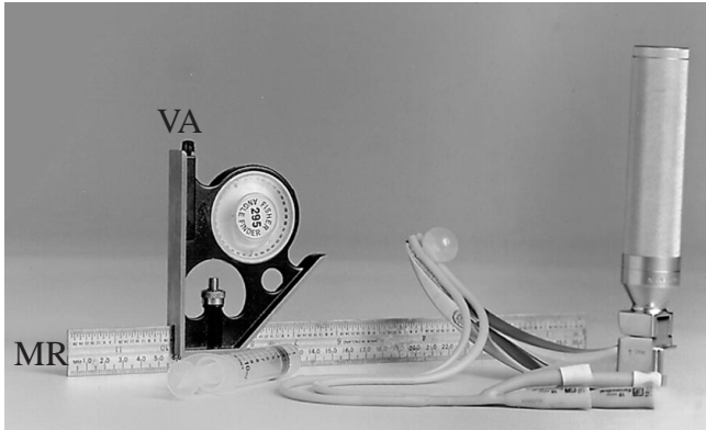
Modified Macintosh Blade with right catheter balloon inflated with 2 ml air and automatic angle finder. MR, angle finder's metallic ruler; VA, angle finder's vertical arm.
