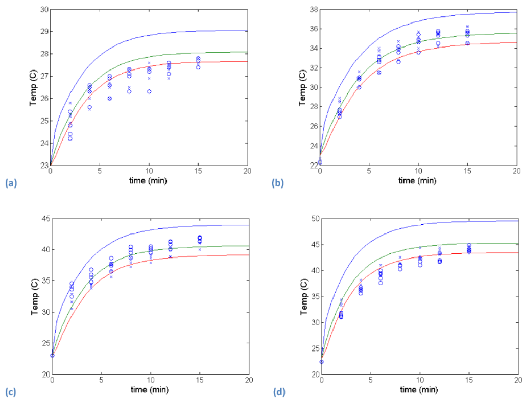
Figure 3. Experimental temperature measurements (2 samples, circles and crosses) and heat transfer model predictions (solid lines for three radial points in the domain) for 4 different ODs - (a) 0.065, (b) 0.148, (c) 0.285, and (d) 0.50.
