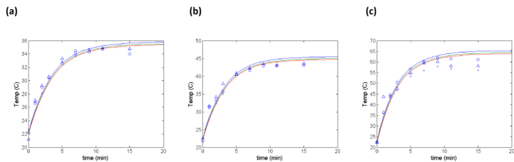
Figure 5. Heat transfer model prediction at different radial locations (solid lines) and experimental temperature measurements (open circles and crosses) at three different laser energy levels -- (a) 0.008 \text{ W/mm}^3 , (b) 0.016 \text{ W/mm}^3 , and (c) 0.032 \text{ W/mm}^3 .
