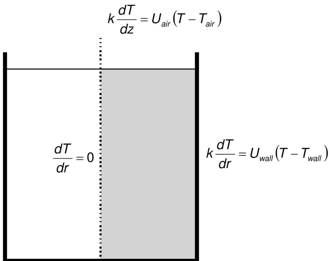
Figure 2. The model domain (grey) represents a symmetrical cross-section of a well in a plate. The top boundary is the air-solution interface, the right and bottom boundaries are plate-solution interfaces, and the left boundary (dotted line) is the symmetry axis.
