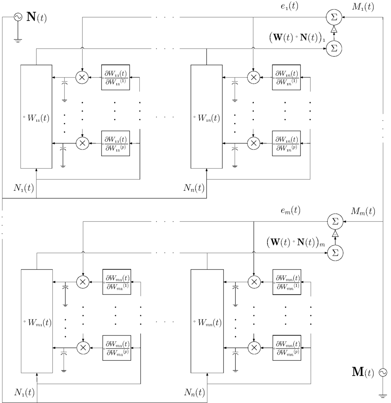
Fig. 1. Block diagram of a computational architecture for linear convolutional decoding and learning.
