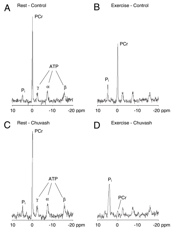
Fig. 2. Examples of spectra obtained from calf muscle during 31 P MRS. (A and B) Spectra for a representative control participant. (C and D) Spectra for a representative CP patient. (A and C) Spectra recorded at rest. (B and D) Spectra recorded in the last minute of the 5-W exercise period. The depletion of PCr and increase in P i with exercise was much more marked in the Chuvash patient than in the control participant.
