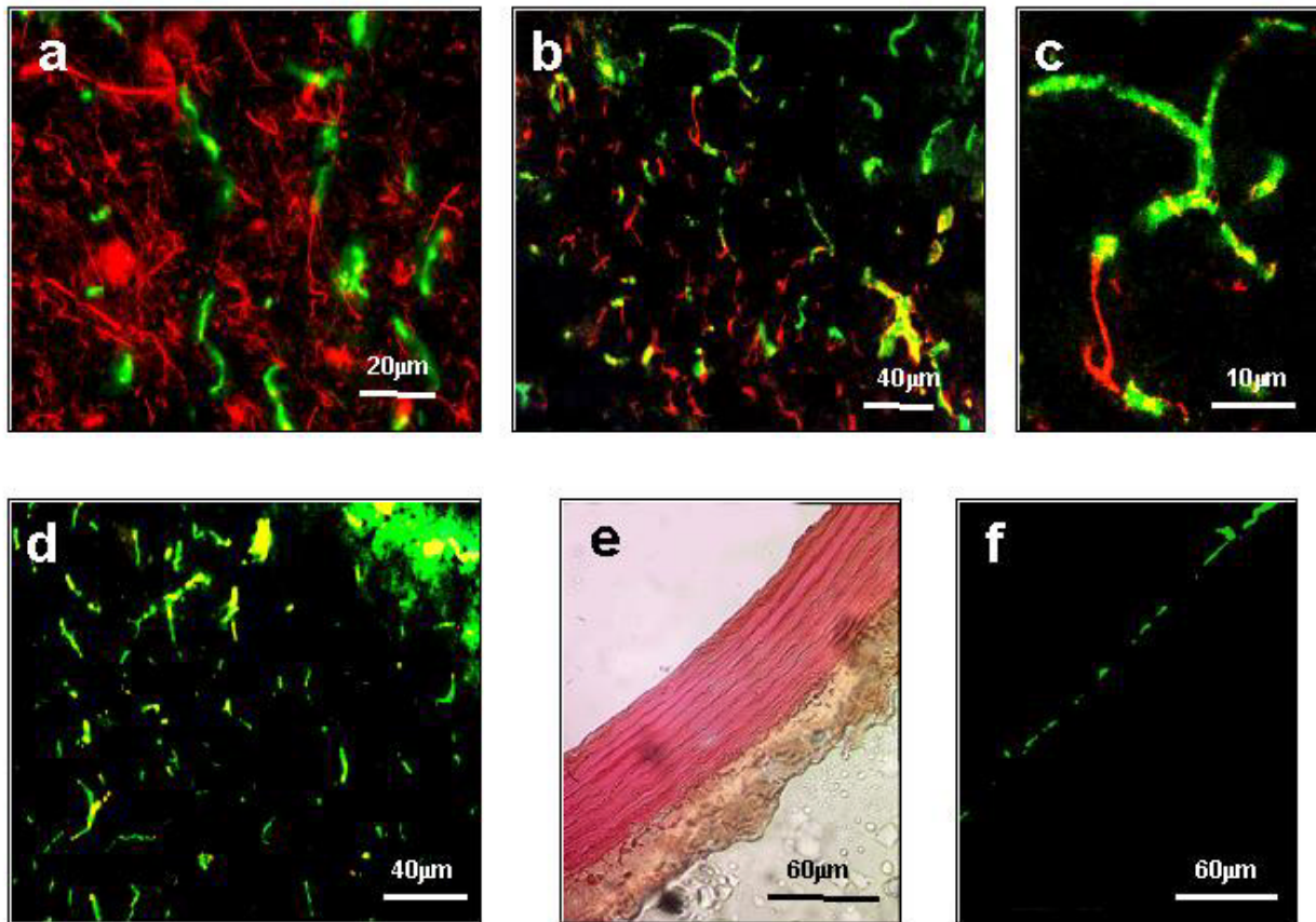
Figure 3 Colocalization of \beta -dystroglycan and von Willebrand factor in normal mouse forebrain. Shown are cryosections indirectly labeled with rhodamine-conjugated antibodies to the neurofilament of apparent 68 kDa (a), the glial fibrillary acidic protein (b, c) and von Willebrand factor (d). Sections (a) to (d) were indirectly double-labeled with a fluorescein-conjugated antibody against \beta -dystroglycan. To demonstrate the specificity of the antibody to von Willebrand factor, rat aorta sections are shown in (e) (Haematoxylin & Eosin staining) and (f) (immunofluorescence labeled). In (a), bar = 20 \mu\text{m} ; in (b) and (d), bar = 40 \mu\text{m} ; in (c), bar = 10 \mu\text{m} ; and in (e) and (f), bar = 60 \mu\text{m} .
