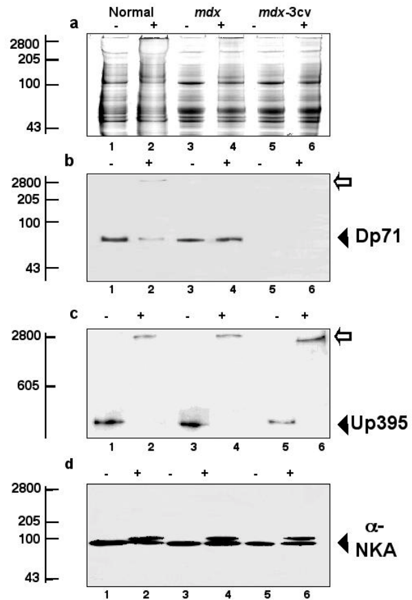
Figure 8 Chemical crosslinking analysis of brain dystrophin isoform Dp71 in normal and mdx mice. Shown is a Coomassie-stained gel (a) and identical immunoblots labeled with antibodies to the dystrophin isoform of apparent 71 kDa (Dp71) (b), full-length utrophin of apparent 395 kDa (Up395) (c), and the \alpha -subunit of the \text{Na}^+/\text{K}^+ -ATPase ( \alpha -NKA) (d). Lanes 1, 3 and 5 represent untreated control samples (-) and lanes 2, 4 and 6 are membranes treated with 200 \mu\text{g} crosslinker \text{BS}^3 per mg protein (+). Lanes 1 and 2, 3 and 4, and 5 and 6 represent microsomal membranes isolated from normal brain, mdx brain, and mdx-3cv brain, respectively. The position of immuno-decorated monomers is indicated by closed arrow heads and crosslinking-stabilized high-molecular-mass complexes marked by open arrows. The relative position of molecular mass standards ( \times 10^{-3} ) is indicated on the left.
