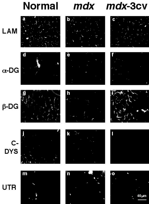
Figure 4 Immunofluorescence localization of \beta -dystroglycan and associated components in forebrain from dystrophic animal models. Shown are cryosections labeled with antibodies to laminin (LAM) (a-c), \alpha -dystroglycan ( \alpha -DG) (d-f), \beta -dystroglycan ( \beta -DG) (g-i), the carboxy-terminus of dystrophin (C-DYS) (j-l), and utrophin (UTR) (m-o). Forebrain specimens were taken from normal mice (a, d, g, j, m), mdx mice (b, e, h, k, n) and mdx-3cv mice (c, f, i, l, o). Bar = 40 \mu m.
