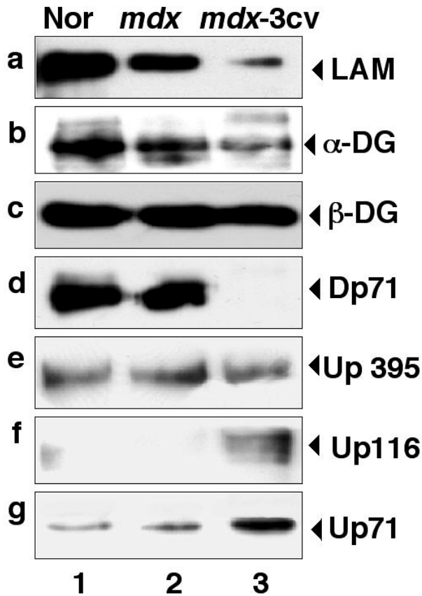
Figure 7 Immunoblot analysis of \beta dystroglycan and associated components in normal and dystrophic brain-membranes. Shown are identical immunoblots labeled with antibodies to laminin (LAM) (a), \alpha -dystroglycan ( \alpha -DG) (b), \beta -dystroglycan ( \beta -DG) (c), dystrophin of apparent 71 kDa (Dp71) (d), full-length utrophin of apparent 395 kDa (Up395) (e), the utrophin isoform of apparent 116 kDa (Up116) (f), and the utrophin isoform of apparent 71 kDa (Up71) (g). Lanes 1 to 3 represent microsomal membranes isolated from normal brain, mdx brain, and mdx-3cv brain, respectively. The position of immuno-decorated protein bands is indicated by arrow heads.
