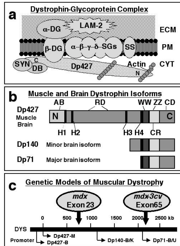
Figure 1 Diagrammatic representation of the dystrophin-glycoprotein complex, the structure of muscle and brain dystrophin isoforms and the genetic animal models of muscular dystrophy. In muscle, dystrophin forms a tightly associated complex with various surface components which provides a stabilizing linkage between the sub-sarcolemmal membrane cytoskeleton and the extracellular matrix. In panel (a) is shown the proposed spatial organization of this peripheral complex consisting of dystrophin (Dp427), \alpha -, \beta -, \gamma -, and \delta -sarcoglycan (SG), the sarcolemma-spanning backbone structure provided by \alpha - and \beta -dystroglycan (DG), sarcospan (SS), various syntrophins (SYN) and dystrobrevins (DB), as well as laminin-2 (LAM-2) and cortical actin. Panel (b) outlines the various domains of dystrophin molecules with the N-terminal actin-binding domain (AB), hinge regions (H), the central spectrin-like rod domain (RD), as well as C-terminal binding domains such as the WW domain, the ZZ domain, the cysteine-rich region (CR) and the extreme carboxy-terminal domain (CD). While skeletal muscle fibres contain the Dp427 isoform of dystrophin, brain tissues express besides the full-length Dp427 molecule also two shorter isoforms termed Dp71 and Dp140 (b). Four of the seven promoters which drive the tissue-specific expression of dystrophins are shown in panel (c) illustrating that a point mutation in exon 23 or a mutation in exon 65 results in the absence of Dp427 in mdx mice and the absence of all brain isoforms of dystrophin in mdx-3cv mice.
