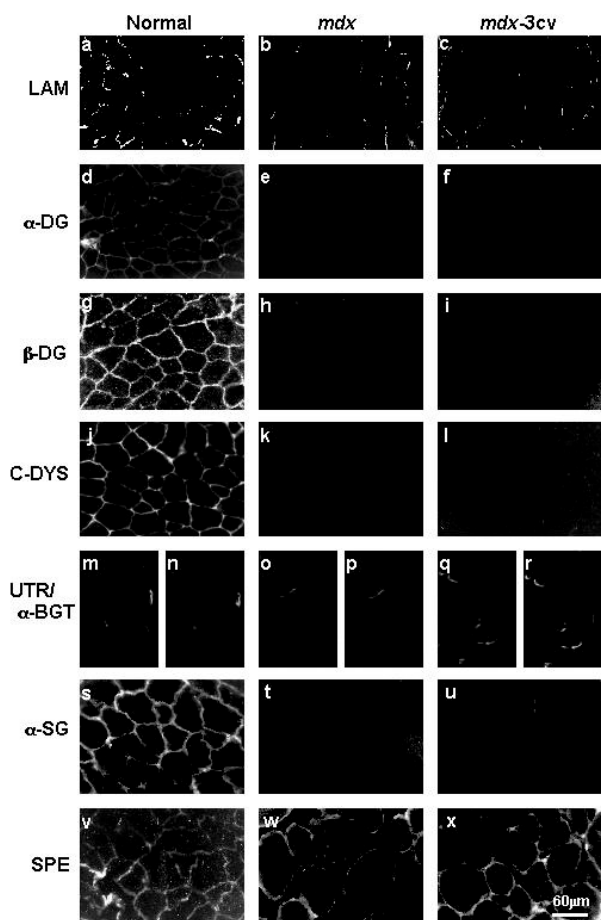
Figure 2 Immunofluorescence localization of \beta -dystroglycan and associated components in skeletal muscle fibres from dystrophic animal models. Shown are cryosections labeled with antibodies to laminin (LAM) (a-c), \alpha -dystroglycan ( \alpha -DG) (d-f), \beta -dystroglycan ( \beta -DG) (g-i), the carboxy-terminus of dystrophin (C-DYS) (j-l), utrophin (UTR) (m, o, q), \alpha -sarcoglycan ( \alpha -SG) (s-u), and spectrin (SPE) (v-x). Panels (n), (p) and (r) represent labeling of tissue sections with \alpha -bungarotoxin ( \alpha -BGT). Skeletal muscle specimens were taken from normal mice (a, d, g, j, m, n, s, v), mdx mice (b, e, h, k, o, p, t, w) and mdx-3cv mice (c, f, i, l, q, r, u, x). Bar = 60 \mu m.
