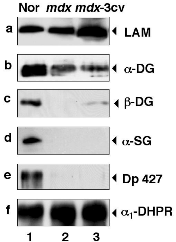
Figure 5 Immunoblot analysis of \beta -dystroglycan and associated components in normal and dystrophic skeletal muscle fibres. Shown are identical immunoblots labeled with antibodies to laminin (LAM) (a), \alpha -dystroglycan ( \alpha -DG) (b), \beta -dystroglycan ( \beta -DG) (c), \alpha -sarcoglycan ( \alpha -SG) (d), full-length dystrophin of apparent 427 kDa (Dp427) (e), and the \alpha_1 -subunit of the dihydropyridine receptor ( \alpha_1 -DHPR) (f). Lanes 1 to 3 represent microsomal membranes isolated from normal muscle fibres, mdx fibres, and mdx-3cv fibres, respectively. The position of immuno-decorated protein bands is indicated by arrow heads.
