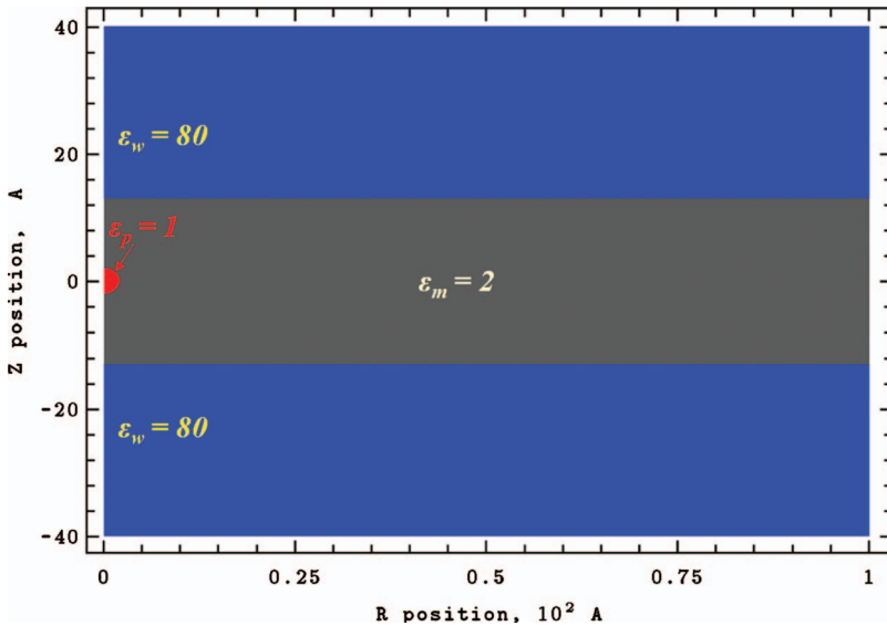
FIG. 1. Two-dimensional cylindrical computational domain with R=100 Å and Z between -40 and 40 Å. This system is multielectric: membrane with dielectric constant \epsilon_m=2 ; the water domains with \epsilon_w=80 and the charged sphere of radius 2 Å with \epsilon_p=1 . A mesh with spacings of 0.1 and 0.2 Å ( 1001 \times 801 and 501 \times 401 grid points) was used in computation. The figure is generated using our CE-MEA code.
