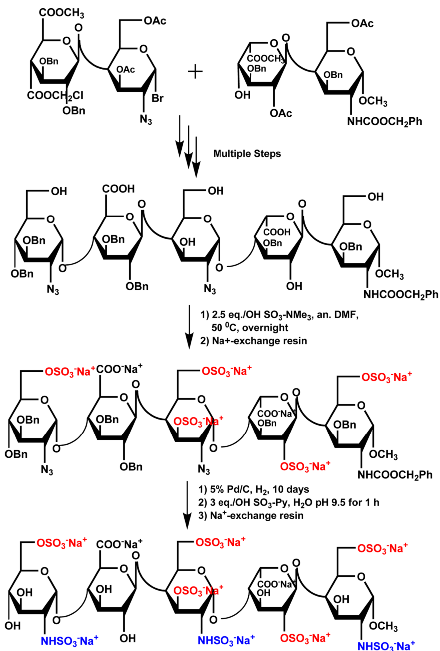
Scheme 2.
