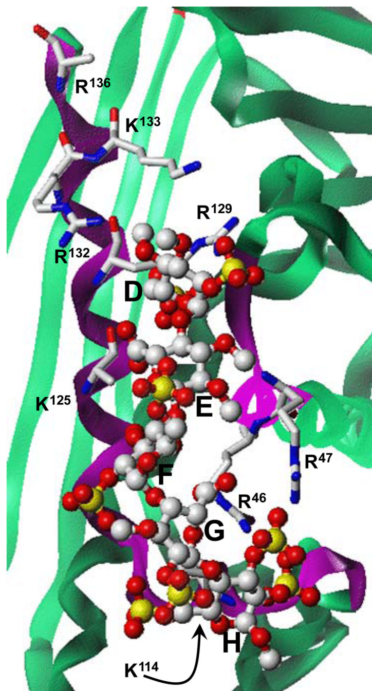
Figure 3. Close-up view of the heparin-binding site in antithrombin
