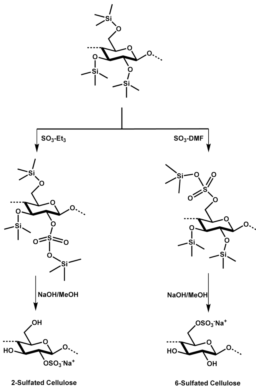
Scheme 12.
