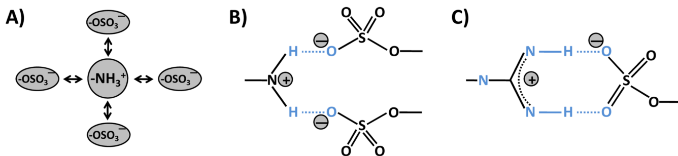
Figure 2. Interaction of sulfate group(s) with positively charged nitrogen containing groups A) The interaction relies solely on the ionic charges on the two groups. This interaction is defined as Coulomb-type interaction and occurs over a longer range in comparison to other atomic interactions. It is isotropic and does not involve any geometrical constraints. B) The interaction between a Lys or an Arg with one or more sulfate groups may sandwich an H atom resulting in the formation of a hydrogen bond. This H-bond may not be linear, yet provides sufficient energy to engineer specificity of recognition. The stoichiometry of interaction here may be 1:1 or 1:2 per nitrogen atom. C) For arginine, a linear H-bond geometry is feasible generating significant bond energy and greater specificity of recognition. The stoichiometry of interaction here is 1:1. Geometry C) is expected to be most stable.
