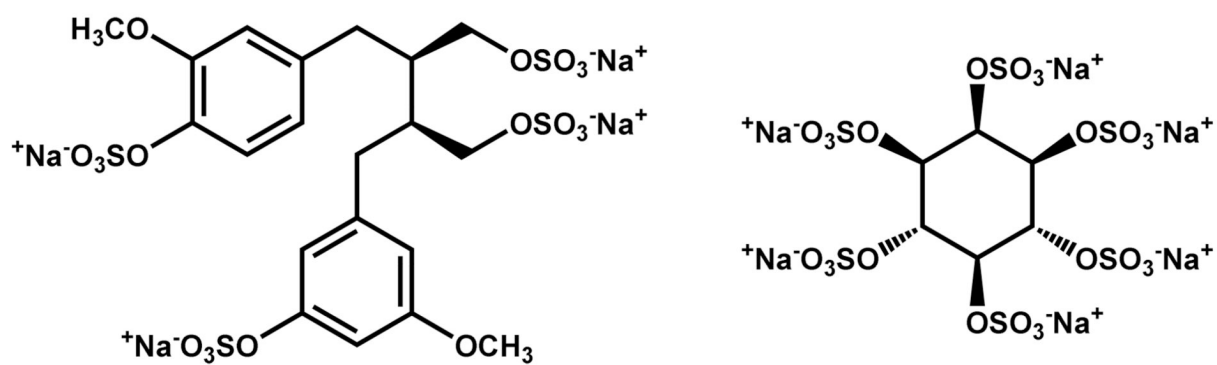
Scheme 5.
