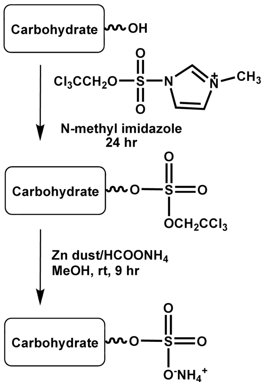
Scheme 9.
