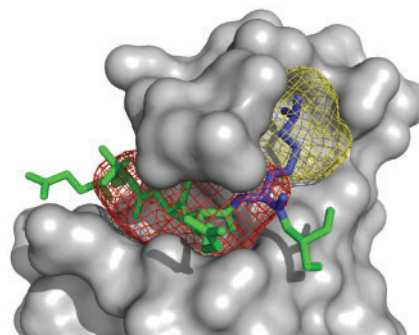
Fig. 1. Sample SITEHOUND output. Chromo domain of HP1 complexed with histone H3 tail (green) containing dimethyl-lysine 9 (blue) (PDB 1kna). SITEHOUND methyl probe clusters are shown as mesh surfaces. The red cluster identifies the peptide-binding region; the yellow cluster identifies the dimethyl-lysine-binding environment. The figure was rendered with PyMOL (DeLano) using the SITEHOUND ‘_clusters.pdb’ output file.
