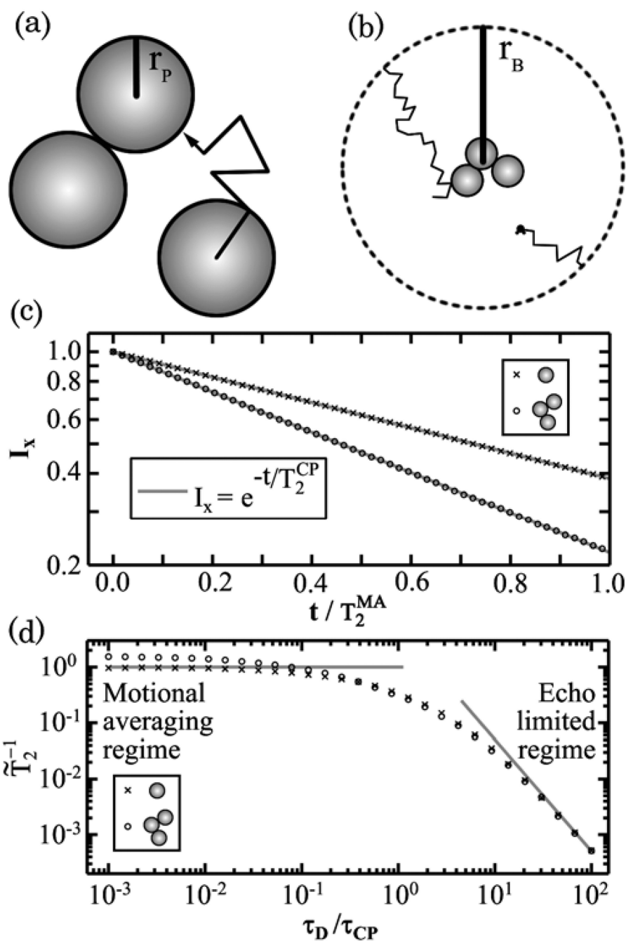
Fig. 1. (a) Schematic diagram showing the diffusion limited aggregation (DLA) of superparamagnetic iron oxide (SPIO) nanoparticles. (b) Illustration of a water molecule executing a random walk in a sphere of radius r_B . (c) Simulated ensemble averaged x-component I_x of water nuclear magnetic moments vs. time t plotted at multiples of 33\tau_{CP} for a single particle and a three-nanoparticle aggregate where \tau_{CP} is the Carr-Purcell-Meiboom-Gill pulse-echo delay time. The size of the points is greater than the statistical error. Linear fits show that both curves are exponential decays. (d) Simulated normalized transverse decay rate \tilde{T}_2^{-1} vs. \tau_D/\tau_{CP} for a single nanoparticle and for a three-nanoparticle aggregate,
