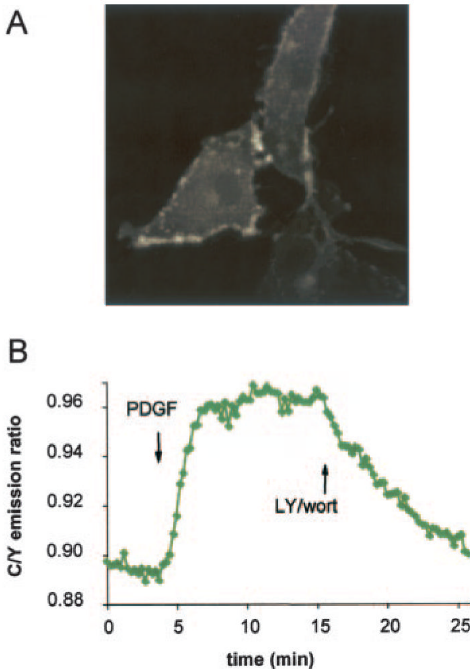
Fig. 4. Membrane targeting of BKAR reveals rapid PKB signaling
