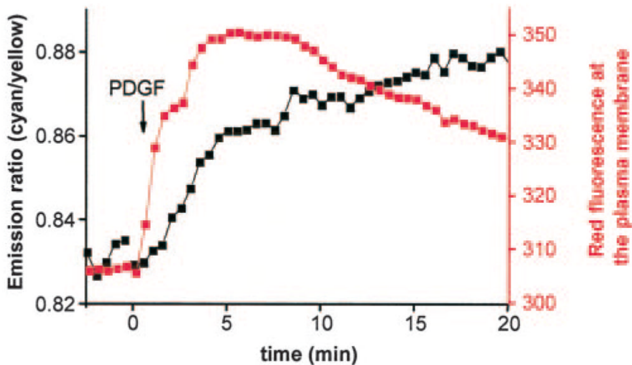
Fig. 5. Simultaneous imaging of PH domain translocation and PKB signaling Serum-starved NIH3T3 overexpressing a monomeric RFP-tagged PKB-PH domain and BKAR were imaged in response to 50 ng/ml PDGF treatment. The intensity of the RFP signal at the plasma membrane ( red ) and the FRET ratio change from cytosolic BKAR ( black ) were assayed concurrently from the same cells and plotted.
