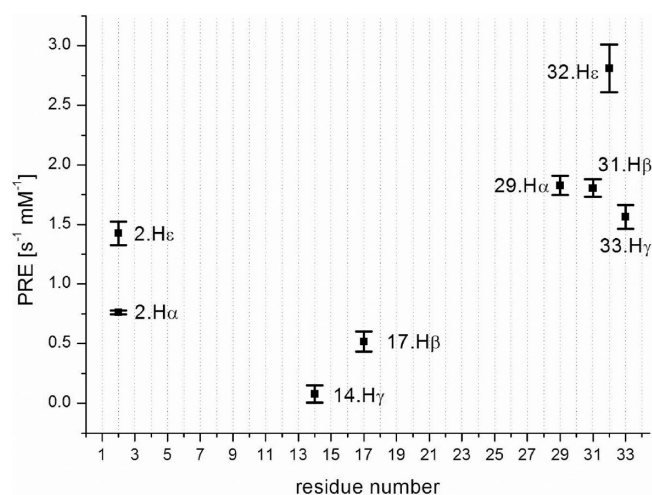
FIGURE 5: Longitudinal ( R_1 ) paramagnetic relaxation enhancements (PREs) of Fst obtained by adding Gd(DTPA-BMA). Only values of well-resolved peaks with correlation coefficients of least-squares fits higher than 0.98 were used. A low PRE is indicative of a larger distance from the micelle surface.
