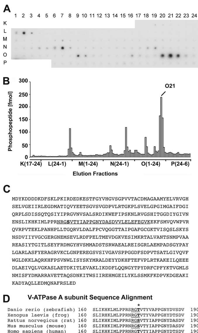
FIGURE 1. Identification of Ser-175 as a major site for PKA phosphorylation in the V-ATPase A subunit. FLAG-A V-ATPase subunit expressed in HEK-293T cells was incubated with a substoichiometric amount of PKA in the presence of [ \gamma - ^{32} P]ATP, the proteins were subjected to SDS-PAGE, and the band corresponding to FLAG-A V-ATPase A-subunit was excised. A , autoradiographic film showing the fractionation profile of phosphopeptide mixtures after in-gel digestion and microfractionation onto prespotted AnchorChips. B , analysis by densitometry of individual radioactive spots identified after the microfractionation (shown in A ) and quantification of the phosphorylated peptides using appropriate standards. The major radioactive peak eluted in fraction E10 and the corresponding phosphorylated peptide was identified by mass spectrometry. C , mouse FLAG-tagged V-ATPase A subunit amino acid sequence highlighting the major peptide phosphorylated by PKA (O21 fraction). D , Ser-175 ( bold ) is part of a highly conserved PKA consensus target phosphorylation site in this peptide.
