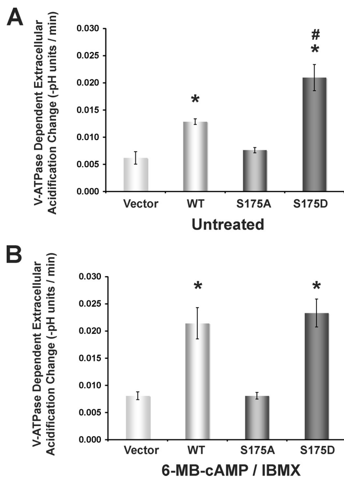
FIGURE 5. Bafilomycin-sensitive, V-ATPase-dependent extracellular acidification is modulated by Ser-175 A subunit mutants and PKA activators in HEK-293T cells. Cells were transfected with vector alone, WT, S175A, or S175D mutant FLAG-tagged A subunit for 28–31 h, and the rate of extracellular acidification in each set of transfected cells was measured in a low buffering capacity solution before and after the addition of bafilomycin A1, a specific V-ATPase inhibitor (see “Experimental Procedures”). The mean ( \pm S.E.) rate of extracellular acidification [-(\text{final buffer pH} - \text{initial buffer pH})/\Delta t] was obtained in the absence or presence of bafilomycin, for cells incubated either with (A) or without (B) PKA activators ( n = 6 for each transfection condition; n = 6 for each treatment condition) (*, p < 0.005 relative to vector alone; #, p < 0.02 relative to WT).
