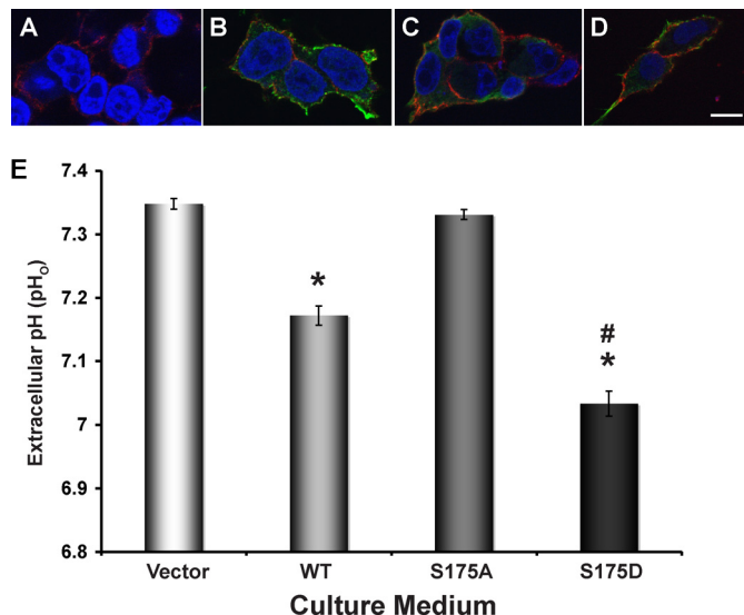
FIGURE 4. Expression of WT and mutant V-ATPase A subunit in HEK-293T cells modulates subcellular localization of the A subunit and extracellular pH. HEK-293T cells were transfected with either vector alone ( A ) or FLAG-tagged WT ( B ), S175A ( C ), or S175D ( D ) mutant A subunit 1 day prior to immunofluorescence staining for expression of FLAG (green), concanavalin A coupled to CY3 as a membrane marker (red), and TO-PRO-3 nuclear stain (blue). Scale bar = 15 μm. E , mean (±S.E.) extracellular pH (pH o ) of the culture medium from HEK-293T cells transfected with different plasmids after 28–31 h incubation (*, p < 0.0001 relative to vector alone; #, p < 0.0001 relative to WT; n = 15–18).
