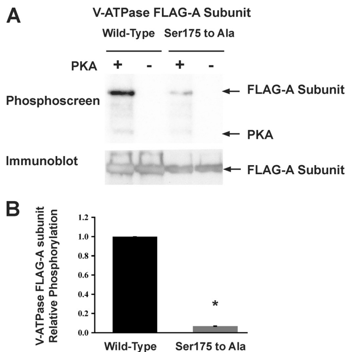
FIGURE 2. PKA phosphorylation of the A subunit in vitro occurs at Ser-175. A , typical phosphoscreen image ( upper ) revealing the signal of PKA in vitro phosphorylated A subunit compared with the Ser-175 to Ala mutant. The immunoblot blot ( lower ) confirms similar protein expression and loading of the gel for the different conditions. B , quantification of mean ( \pm S.E.) V-ATPase A subunit phosphorylation signal normalized for protein loading as assessed by densitometry of Western blot. Compared with WT FLAG-A subunit, the phosphorylation-deficient (Ser to Ala) mutant showed a significant 90–95% decrease in phosphorylation by PKA in vitro (*, p < 0.05 relative to WT; n = 3 ).
