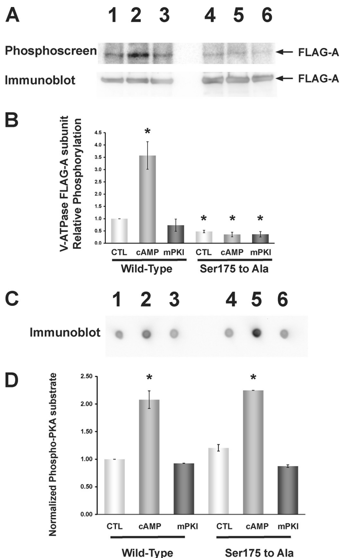
FIGURE 3. PKA-dependent in vivo phosphorylation of the V-ATPase A subunit in HEK-293T cells occurs at Ser-175. FLAG-tagged WT or S175A mutant A subunit was transfected into HEK-293T cells 1 day before experimentation, and cells were then incubated with [ 32 P]orthophosphate for 2 h under control conditions or in the presence of PKA activator (1 mM 6-MB-cAMP; last 20 min of labeling period) or PKA inhibitor (10 μM mPKI; for entire labeling period). Cell lysis, immunoprecipitation using an anti-FLAG antibody, SDS-PAGE, immunoblotting using an anti-FLAG antibody, and exposure of the same membrane to a phosphoscreen were then performed as described (38). A , typical phosphoscreen image (upper panel) revealing the signal of phosphorylated A subunit in cells expressing FLAG-A-WT subunit (lanes 1–3) or FLAG-A-S175A subunit (lanes 4–6). Lanes 1 and 4 were derived from control-treated cells, lanes 2 and 5 were derived from PKA-stimulated cells, and lanes 3 and 6 were derived from PKA-inhibited cells. The Western blot (lower panel) confirms similar protein expression and loading of the gel for the different conditions. B , quantification of mean (±S.E.) V-ATPase A subunit phosphorylation signal relative to FLAG-A-WT control condition and normalized for protein expression. PKA activator increased FLAG-A-WT phosphorylation to ~3.5 times that of the control condition, whereas FLAG-A-S175A mutant subunit phosphorylation was reduced across all conditions to ~0.5 times that of the FLAG-A-WT subunit under the control condition (*, p < 0.05 relative to WT control by analysis of variance; n = 3 replicate experiments). C , dot blots using the PKA phosphorylation substrate-specific antibody of whole cell lysate samples taken from cells transfected and treated under the same conditions as shown in A and B and spotted onto a nitrocellulose filter. D , quantification of mean (±S.E.) PKA-phosphorylated substrate signal relative to that FLAG-A-WT-transfected cell lysates under the control condition and normalized to β-actin blot signal re-probed on the same dot blot (not shown). PKA activator 6-MB-cAMP increased the PKA-phosphorylated substrate signal to 2–2.5 times that of control (*, p < 0.05, relative to FLAG-A-WT
