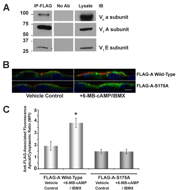
FIGURE 6. The phosphorylation-deficient V-ATPase A subunit Ser-175 to Ala mutant does not accumulate at the apical membrane of intercalated cells in response to PKA activators. The Clone C cell line of intercalated cell characteristics was used for independent transient transfections using either WT or S175A A subunit. A , immunoprecipitation using an anti-FLAG antibody (IP-FLAG; left column) followed by immunoblotting using antibodies against the a (upper), A (middle), or E (lower) V-ATPase subunits revealed that the transfected FLAG-tagged A subunit forms a complex with the native V_o sector a subunit and with the V_1 sector E subunit. No co-immunoprecipitation was observed when no antibody was added to the immunoprecipitation reaction (center column). Samples of the whole cell lysate (5%) were also directly immunoblotted for each of the three subunits (right column). B , 1 day after transfection with either FLAG-A wild-type subunit (top panels) or FLAG-A S175A mutant subunit (lower panels), Clone C cells were plated onto Transwell filters. After 4 days the filters were incubated in PBS, pH 7.1, with 100 \mu\text{M} 6-MB-cAMP and 0.5 mM IBMX (right panels) or with PBS, pH 7.1, alone (left panels) for 30 min. These incubations were followed by an incubation with concanavalin A coupled to CY3 (red) for 5 min in PBS, pH 7.1, fixation, and immunofluorescence labeling using anti-FLAG antibody (green) and TO-PRO-3 nuclear stain (blue). Scale bar = 10 \mu\text{m} . C , quantification of V-ATPase-associated mean pixel intensity (MPI) ratio of apical ROI-1 (where the A-subunit co-localizes with concanavalin A) and cytoplasmic ROI-2 (A-subunit alone). This ROI-1/ROI-2 ratio under the different conditions reveals a significant PKA-mediated apical V-ATPase accumulation in cells expressing the WT A subunit compared with cells expressing the S175A mutant (ROI-1/ROI-2 ratio presented as mean ( \pm S.E.); *, p < 0.05 versus V-ATPase A WT; n = 20 –45 cells analyzed for both conditions).
