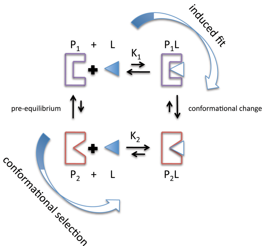
Figure 1. Thermodynamic cycle for molecular recognition processes involving induced fit or conformational selection. In conformational selection, the binding competent conformation (red, P_2 ) is pre-existing in solution prior to the addition of ligand ( L ). The kinetic and thermodynamic rate constants can determine if conformational selection or induced fit is more likely 8,99
