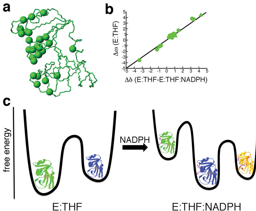
Figure 2. Conformational selection in protein-ligand interactions observed by NMR R_2 relaxation dispersion experiments. (a) Locations of conformational exchange are indicated as spheres on the structure of DHFR (pdb 1rx5). (b) A linear correlation between \Delta\omega (chemical shift difference between ground-state and higher energy conformations) from R_2 relaxation dispersion experiments of the product binary complex of DHFR (enzyme bound with tetrahydrofolate (E:THF)) and \Delta\delta from ground-state chemical shift differences between product binary and ternary (enzyme bound with tetrahydrofolate and NADPH cofactor (E:THF:NADPH)) complexes indicate that the higher energy conformation of the product binary complex is structurally similar to the ground-state of the product ternary complex (i.e. chemical shifts of the higher energy conformation of the product binary complex are similar to the chemical shifts of the ground-state conformation of the product ternary complex) (data taken from ref41). (c) The binding of the NADPH cofactor changes the free energy landscape of the enzyme. Structurally similar conformations are colored alike.
