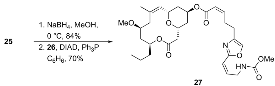
Scheme 10. Synthesis of dehydroneopeltolide.
