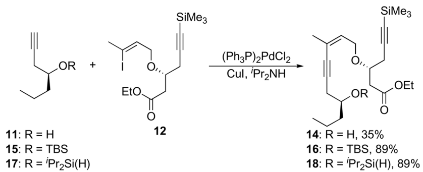
Scheme 5. Sonogashira coupling.
