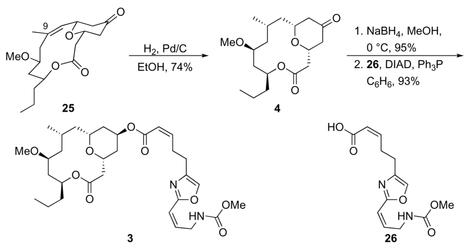
Scheme 9. Synthesis of neopeltolide.
