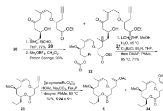
Scheme 7. Completion of the cyclization substrate synthesis.
