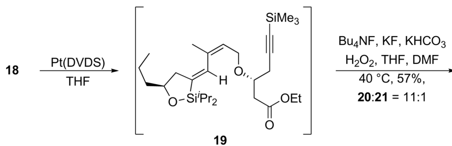
Scheme 6. Alkyne hydration through hydrosilylation.
