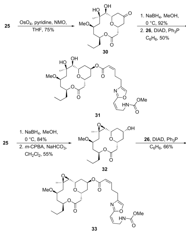
Scheme 12. Synthesis of dihydroxy- and epoxyneopeltolide.
