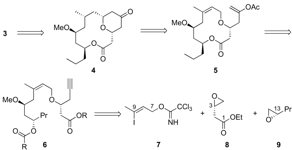
Scheme 2. Retrosynthetic analysis of neopeltolide.
