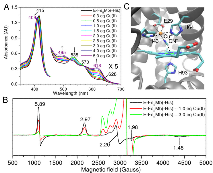
Figure 1. (A) UV-vis titration of ferric E-Fe B Mb(-His) with Cu(II) in 25 mM KH 2 PO 4 , 75 mM KCl, pH 7.0, 25 °C; (B) X-band EPR spectra of ferric EFe B Mb(-His) (0.5 mM) in the same buffer as in (A) and that in the presence of 1.0 or 3.0 eq Cu(II). The spectra were collected at 20 K, 5 mW power, and 9.05 GHz; (C) Crystal structure of Cu(II)-CN - -Fe B Mb(-His) at 1.65 Å resolution (PDB entry 3MN0).
