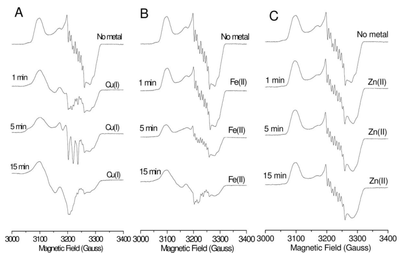
Figure 2. EPR spectra of deoxy E-Fe B Mb(-His) (0.5 mM) in the presence of NO after 5 min (top line), with 2 eq Cu(I) (A), Fe(II) (B) or Zn(II) (C) incubated with NO for 1 min, 5 min, and 15 min. Spectra were collected in 50 mM Bis-Tris pH 7.0 at 30 K, 0.2 mW power, and 9.05 GHz.
