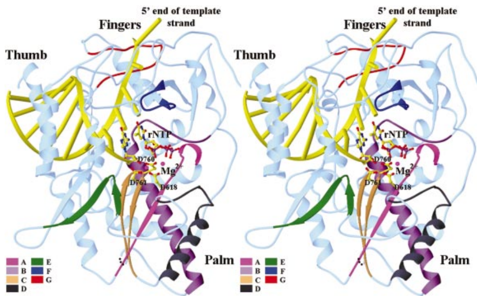
Figure 3. Stereoview of the polymerase active site and the rNTP-binding site. The conserved sequence motifs (A–G) are highlighted. A docked rNTP substrate is shown as a ball-and-stick model. The catalytic active site is defined by the three conserved aspartates, Asp618, Asp760 and Asp761 (shown with side chains) that are coordinated with two divalent metal ions (shown as magenta spheres).
