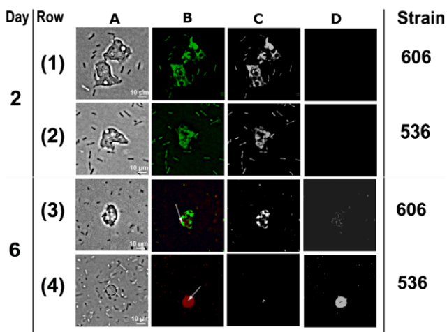
Figure 2. Visualization of the E. coli / D. discoideum viability. (A) Phase contrast microscopy (20×). (B) Combined Red and Green: Green fluorescent stain reflect living cells, red fluorescence reflect cells with damaged membranes. (C) Green channel alone. (D) Red channel alone: (1) Amoeba with the strain E. coli B REL 606 two days after plating, all cells are green reflecting living cells. (2) Amoeba with the strain E. coli 536 two days after plating, all cells are green reflecting living cells. (3) Amoeba with the strain E. coli B REL 606 six days after plating, red fluorescent bacteria are cells with damaged membranes (white arrow), green fluorescent cells are alive (amoeba and bacteria). (4) Amoeba with the strain E. coli 536 six days after plating, green fluorescent bacteria are alive cells (white arrow), red fluorescent amoeba and bacteria are cells with damaged membranes. doi:10.1371/journal.pone.0011882.g002
