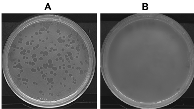
Figure 3. Bacterial lysis plaque occurrence. (A) A non-virulent E. coli strain (B REL606; 10^8 cells) was plated with D. discoideum ( 10^2 cells). Bacterial lysis plaques were observed, characteristic of the grazing phenotype. (B) A virulent E. coli strain (536; 10^8 cells) was plated with D. discoideum ( 10^2 cells). No bacterial lysis plaques were observed, characteristic of the grazing resistance phenotype. doi:10.1371/journal.pone.0011882.g003
