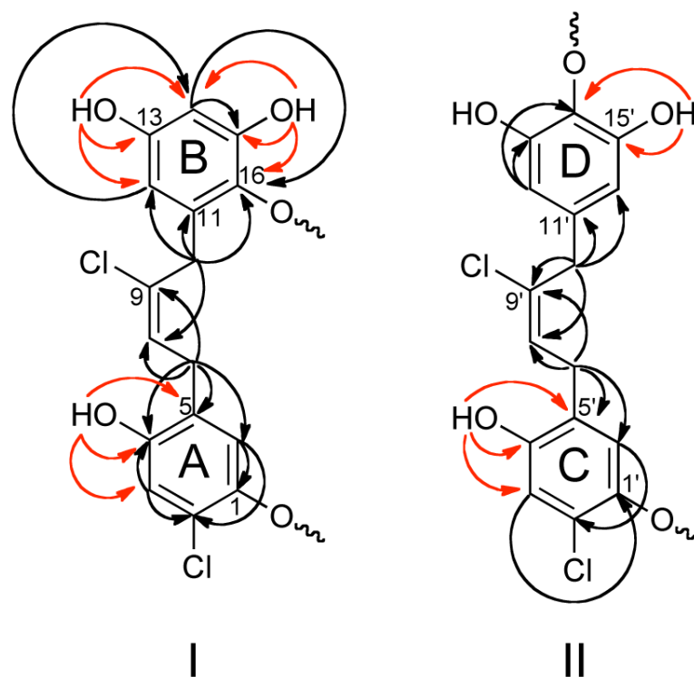
Figure 1. Key HMBC correlations used to establish partial structures corresponding to fragments I and II in compound 1 . ^1\text{H} - ^{13}\text{C} and \text{OH} - ^{13}\text{C} correlations are shown by black and red arrows, respectively.
