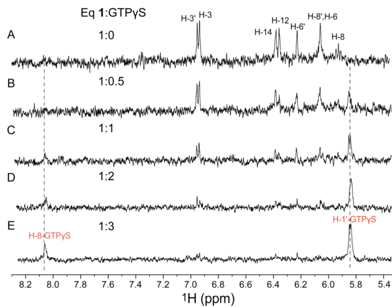
Figure 5. Competition of chrysopaentia A and GTP \gamma S binding to FtsZ by STD NMR. (a) Expanded ^1\text{H} STD NMR spectrum of chrysopaentia A (1.25 mM) in the presence of FtsZ (12.5 \mu\text{M} ). (b-e) STD NMR spectra recorded on the same sample after addition of (b) 0.5, (c) 1.0, (d) 2.0 and (e) 3.0 eq GTP \gamma S. Final concentrations of GTP \gamma S were 625 \mu\text{M} , 1.25 mM, 2.50 mM and 3.75 mM, respectively.
