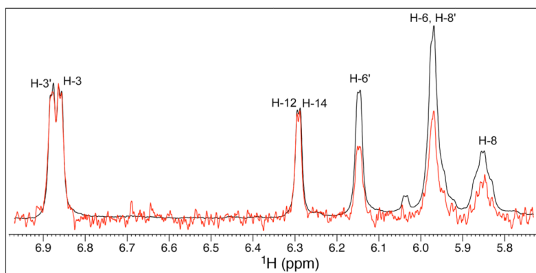
Figure 4. Reference (black) and STD NMR difference (red) spectra of chrysopaentín A in complex with FtsZ. Spectral expansion shows non-overlapped aromatic and olefinic signals of 1 displaying the strongest enhancements upon binding to FtsZ. Samples comprising 100:1 1 :FtsZ were prepared in 20 mM NaPO 4 , 50 mM NaCl, 5 mM MgCl 2 , pH 6.8, and spectra recorded at 298 K. Overlaid spectra were normalized to the signal for H-3 ( \delta 6.85), which gave the strongest enhancement.
