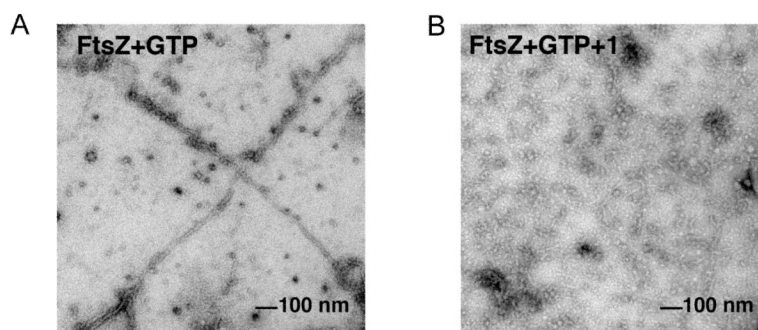
Figure 3. Transmission electron micrographs of FtsZ in the presence of (A) GTP, and (B) GTP and chrysopaentin A. (A) Polymerization of recombinant E. coli FtsZ was induced with addition of GTP for 5 min at rt before transferring to a carbon grid, staining with 3% uranyl acetate, and visualizing by TEM, 44 000 x. (B) Incubation of FtsZ with 1 (50 \mu M) prior to addition of GTP inhibits polymerization and protofilament formation. No filaments were observed over the entire grid shown in panel B.
