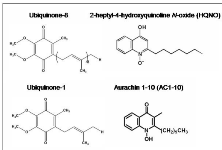
Figure 2. Structures of quinone substrates and quinone-like inhibitors referred to in the text.
