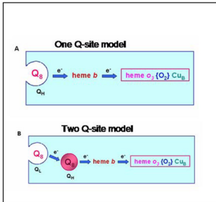
Figure 1. Schematic illustrating the 1-site and 2-site models for quinone binding to cytochrome bo_3 .
