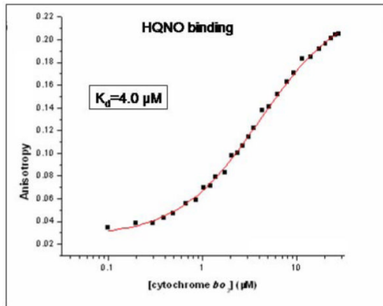
Figure 5. HQNO binding to cytochrome bo 3 which has been isolated with one equivalent of ubiquinone-8 bound to the Q H -site. Binding is monitored by fluorescence anisotropy, titrating the enzyme into a solution containing 1 μM HQNO. The points are experimental data and the line is a fit to 1 binding site with a K d of 4 μM.
