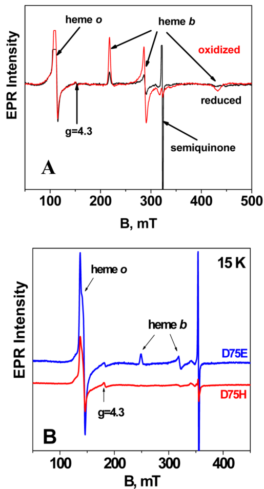
Figure 8. (A) Continuous-wave X-band EPR spectrum of oxidized (red) and reduced (black) cytochrome bo 3 (see text for details). (B) EPR spectra of the reduced D75E and D75H mutants. Temperature 15 K, microwave power ~ 10 mWatt, modulation amplitude 0.5 mT, reduction time 6 hours.
