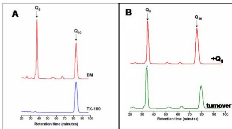
Figure 3. HPLC elution profiles following extraction of ubiquinone-8 from purified cytochrome bo_3 . A known amount of ubiquinone-10 is included in each sample as an internal standard. Panel A: Enzyme isolated in dodecylmaltoside (DM) contains 1 equivalent of ubiquinone-8, whereas enzyme washed with Triton X-100 has no bound ubiquinone-8. Panel B: Enzyme incubated with oxidized ubiquinol-1 ( 500 \mu\text{M} ) retains bound ubiquinone-8 (top), as does enzyme which has been incubated under conditions of catalytic turnover with ubiquinol-1 (see text).
