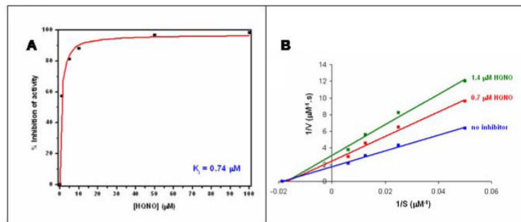
Figure 4. Inhibition of steady state ubiquinol-1 oxidase activity by HQNO. Panel (A) is a direct plot of the data, and Panel (B) is a Lineweaver-Burke plot showing noncompetitive inhibition.
