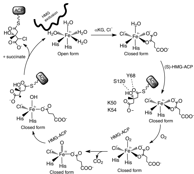
Fig. 3. Hal mechanism and role for conformational change. The resting enzyme ( upper left ) is in the open form and ( S )-HMG-ACP is excluded. \alpha KG and \text{Cl}^- binding trigger the switch to the closed form, to which ( S )-HMG-ACP can bind. Substrate binding permits dioxygen to coordinate the \text{Fe}^{2+} , and triggers oxidative decarboxylation of \alpha KG and formation of the chloro-oxo-ferryl intermediate. The intermediate abstracts a hydrogen atom from the substrate, and the substrate radical is resolved by chlorination via a “rebound” mechanism (13).
