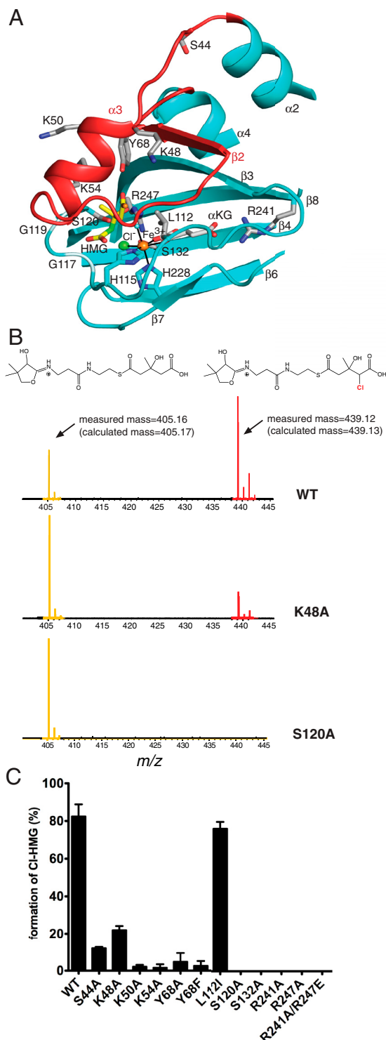
Fig. 4. HMG model and site-directed mutagenesis of Cur Hal. (A) Model of HMG binding in the active site. Residues in contact with modeled HMG (yellow C) include Ser120 to the 3- S -hydroxyl, Tyr68 to the thioester carbonyl and the backbone at residues 117–119 to a carboxylate oxygen. The C4 atom of HMG to be chlorinated is green. Side chains of residues tested by mutagenesis are shown with gray C. (B) PPant-ejection assay of Hal activity. Substrate and product were ejected from ACP by IRMPD and detected by FTICR-MS. HMG-PPant is at m/z 405.16. Cl-HMG-PPant is at m/z 439.12. (C) Activity of wild-type and Hal mutants. Activity is represented as the percent of chlorinated product compared to total species ejected. Each reaction was performed at least in triplicate. Error bars represent the standard error of measurement.
