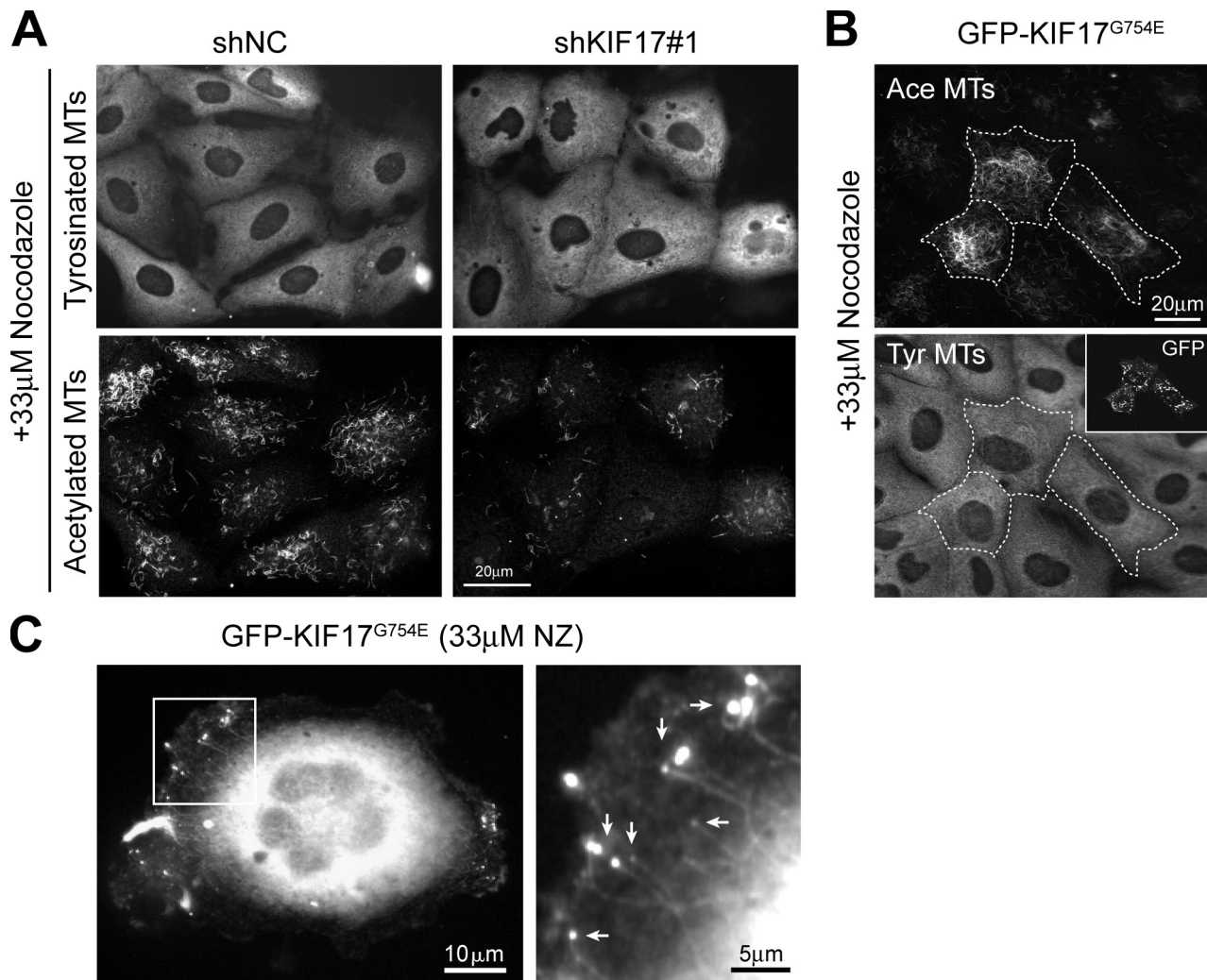
Figure 9. KIF17 affects MT stabilization in epithelial cells. (A) Immunostaining of tyrosinated and acetylated tubulin in MDCK cells infected with shNC or shKIF17#1 and treated for 45 min with 33 \mu M NZ. (B) Acetylated and tyrosinated tubulin in MDCK cells (outlined cells and inset), treated for 1 h with 33 \mu M NZ. (C) Caco2 cells injected with GFP-KIF17 G754E cDNA and treated for 15 min with 33 \mu M NZ. An enlargement of the boxed region is shown on the right. Arrows point to GFP-KIF17 G754E at the ends of NZ-resistant MTs.
