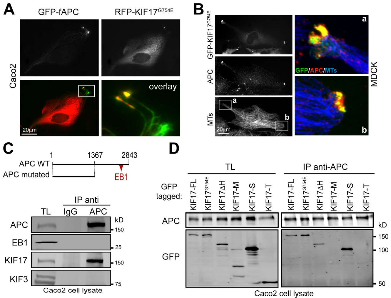
Figure 5. KIF17 coiled-coil region binds APC independently of EB1. (A) Colocalization of GFP-f-APC and mRFP-KIF17 G754E at plus ends of a subset of MTs in Caco2 cells 3 h after cDNA injection. The boxed region is magnified on the right. (B) Immunostaining of APC and tyrosinated tubulin in MDCK cells expressing GFP-KIF17 G754E . Color overlays (a and b) show magnifications of the boxed regions. (C) Schematic of wild-type (WT) and C-terminally truncated APC present in Caco2 cells. The red arrowhead shows the EB1 binding site, which is missing in Caco2 APC. Immunoblots show endogenous APC, EB1, KIF17, and KIF3 in total lysates (TL) and immunoprecipitates from Caco2 cells incubated with rabbit IgG or anti-APC IgG. Numbers on top indicate amino acid position. (D) Immunoblots showing total lysates and immunoprecipitated APC (endogenous) and GFP-KIF17 constructs expressed in Caco2 cells.
