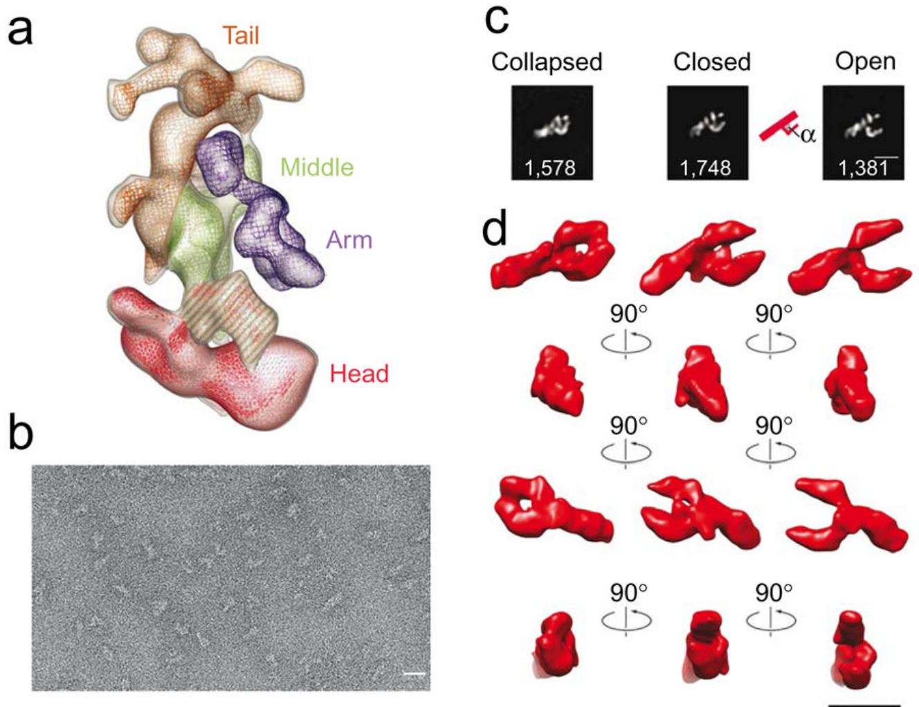
Figure 1. Mediator and Head module structure. (a) A cryo-EM reconstruction of Mediator shows the overall structure of the complex at \sim 25\text{-}\text{\AA} resolution. Previous biochemical, functional and structural analyses suggest a modular organization of Mediator. The Head, Middle/Arm and Tail structural modules have been identified by comparing structures of Mediator in different conformations. A portion of the structurally defined Head module (dashed in green) comprises density corresponding to subunits biochemically identified with the Middle module. (b) A micrograph showing single Head module particles preserved in uranyl acetate. Scale bar, 200 \text{\AA} . (c) Three different conformations of the Head module were identified through reference-free alignment and classification of EM images. Head module particles were nearly evenly distributed among the three different conformations that differ in the position of a smaller corner-shaped domain on the bottom-right of the structure. The angle ( \alpha ) between the larger and smaller portions of the Head module structure (see diagram) is <90^\circ in the collapsed conformation, \sim 90^\circ in the closed conformation and >90^\circ in the open conformation. Information from images of tilted particles was used to obtain 3D reconstruction of the Head module in all three different conformations. Scale bar, 100 \text{\AA} . (d) Different views of Head module volumes in the collapsed (left column), closed (middle column) and open (right column) conformations. Scale bar, 100 \text{\AA} .
