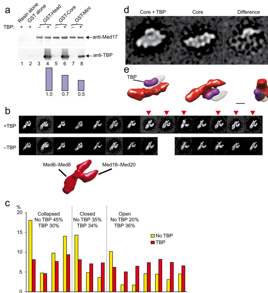
Figure 3. Head-TBP interactions. (a) A GST pull-down assay was used to measure the interaction between TBP and the Head, Core and Mini complexes. GST fusion complexes (as indicated) were immobilized on a glutathione-agarose resin incubated in the presence (lanes 4, 6 and 8) or absence (lanes 3, 5 and 7) of TBP. Controls are shown in lanes 1 and 2. Values for relative TBP binding to the different complexes are represented by the bars below the immunoblot. (b) Class averages obtained after incubation of the Head module with (top) and without TBP (bottom). Interaction with TBP had no effect on the range of conformations adopted by the Head module. (c) TBP interaction influences the distribution of particles among the different conformations of the Head module. The order of groups in the histogram is derived from the order of class averages in b . (d) Class averages calculated from images of Core particles alone (middle) and after incubation with TBP (left), and the difference between them (right). (e) An approximate 3D model of the Head-TBP complex based on the Core + TBP 2D class average and the 3D structure of the Head module. The Core portion of the Head module is shown in red, density corresponding to subunits Med18 and Med20 is represented as a gray mesh, and TBP is shown as a purple surface calculated by low-pass filtering the X-ray structure of TBP 33 .
