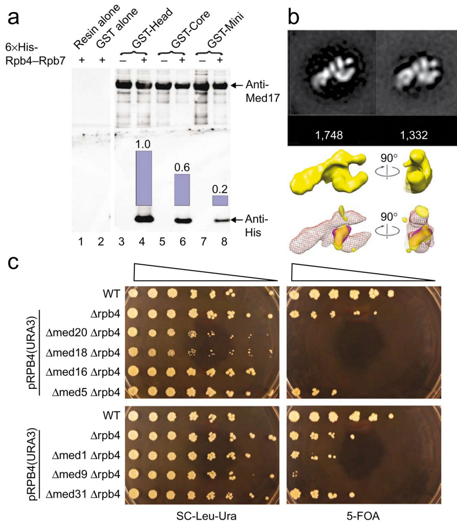
Figure 4. Head module-Rpb4-Rpb7 interaction. (a) A GST pull-down assay was used to measure the interactions between Rpb4-Rpb7 and the Head, Core and Mini complexes. GST fusion complexes (as indicated) were immobilized on glutathione-agarose resin incubated in the presence (lanes 4, 6 and 8) or absence (lanes 3, 5 and 7) of recombinant 6×His-Rpb4-Rpb7. Controls are shown in lanes 1 and 2. Values for relative binding to the different complexes are represented by the bars below the immunoblot. (b) Comparison of class averages obtained after alignment of Head alone (left, 1,748 images) and Head-Rpb4-Rpb7 particles (right, 1,332 images) shows the presence of additional density in the region corresponding to the jaws of the Head module. A 3D reconstruction of the Head-Rpb4-Rpb7 complex (solid yellow surface, right panel top) shows density (semitransparent yellow surface, right panel bottom) matching the size and shape of a low-resolution model calculated from the Rpb4-Rpb7 X-ray structure 32 (purple surface, right panel bottom). (c) Genetic interaction between Rpb4 and Mediator subunits in the Head (Med18 and Med20), Middle (Med1, Med9 and Med20) and Tail (Med16 and Med5) modules was tested by assessing the viability of the synthetic double mutant strains as described in Online Methods. The wild-type (WT) and mutant strains were grown in SC -Leu medium, spotted in five-fold dilutions onto SC -Ura-
