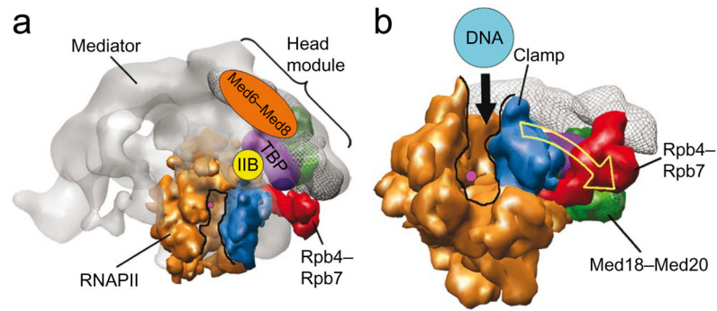
Figure 5. Interaction of the Head module with components of the mPIC and a possible mechanism for initiation regulation. (a) Positioning TBP (shown as a purple surface calculated by low-pass filtering the X-ray structure of TBP) in its approximate binding location to the Head module (adjacent to the Med8 subunit) places the transcription factor in a position matching that predicted by current models of the minimal preinitiation complex structure. This positioning suggests how interaction of RNAPII (shown in orange) with Mediator in the Mediator–RNAPII holoenzyme structure (shown in gray) might help stabilize the preinitiation complex. The magenta circle denotes the approximate position of the RNAPII active site. (b) Interaction of the Head module with the Rpb4–Rpb7 polymerase subunit complex (shown in ruby) documented in this study could be important for enabling Mediator and the general transcription factors to affect the conformation of the polymerase clamp domain (shown in blue), possibly facilitating opening (as indicated by the yellow arrow) of the RNA polymerase II active-site cleft (outlined in black) to allow access of double-stranded promoter DNA to the polymerase active site.
