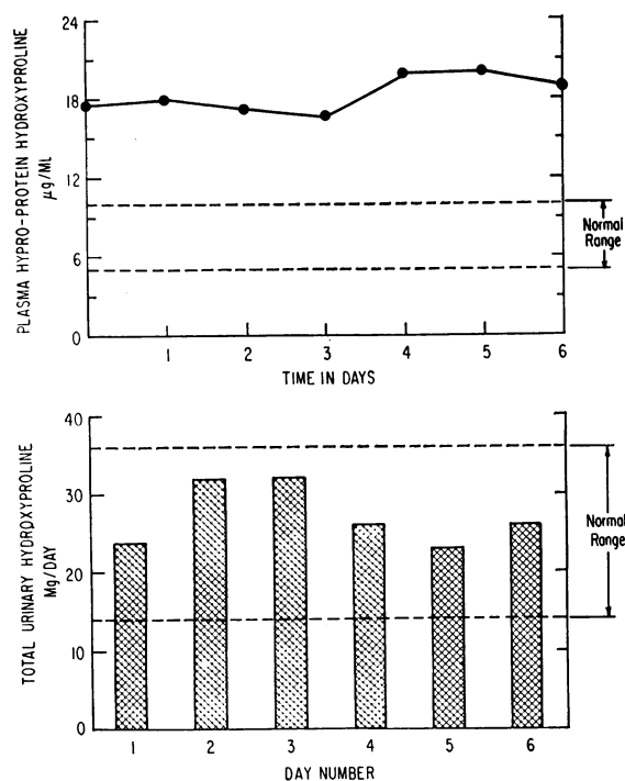
FIG. 3. COMPARISON OF PLASMA HYPROPROTEIN LEVELS WITH URINARY HYDROXYPROLINE PEPTIDE EXCRETION. Two hospitalized adult males with Hodgkin's disease received a hydroxyproline-free diet beginning on the day before the collection of six consecutive 24-hour urine specimens. Daily fasting blood samples were obtained for plasma hyproprotein levels. The data presented are the averages of determinations in the two patients.
