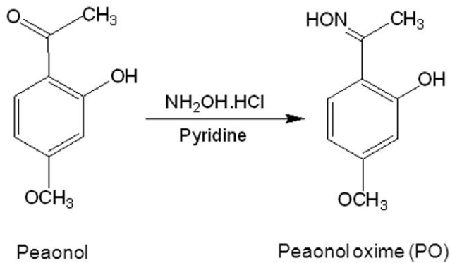
Figure 1. Chemical structure of peonol oxime. Peonol oxime (PO) (1-[2-hydroxy-4-methoxy phenyl] ethanone oxime) was synthesized from peonol. doi:10.1371/journal.pone.0012358.g001
