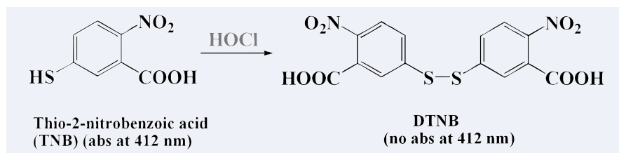
Fig. 14 Detection of HOCl by DTNB.
