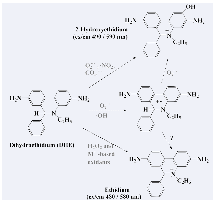
Fig. 5 Structures of DHE, EOH and ethidium and hypothesized reaction pathways to account for the formation of DHE-derived red fluorescence. EOH is basically formed from superoxide and possibly involving \text{ONOO}^-/\text{CO}_2 while ethidium is mainly formed from \text{H}_2\text{O}_2 pathways involving metal proteins. Dotted arrows indicate possible intermediate pathways involved in the formation of these products.
