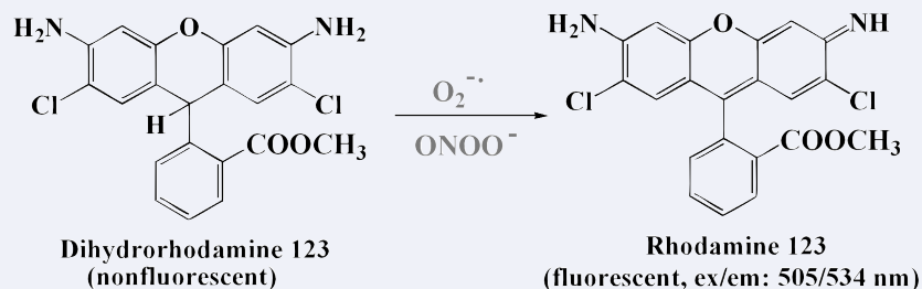
Fig. 7 Detection of \text{ONOO}^- and superoxide by DHR123.
