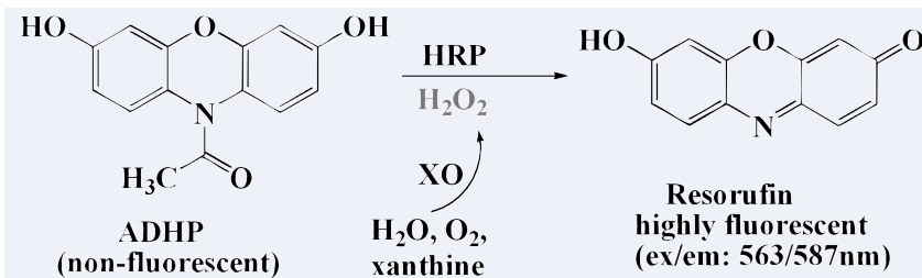
Fig. 11 10-acetyl-3,7-dihydroxyphenoxazine (ADHP) fluorescent assay of XO activity.
