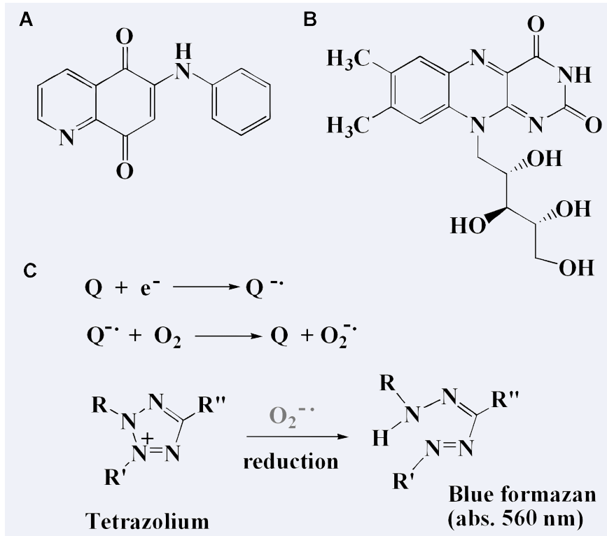
Fig. 3 Structure of quinones (Q): LY83583 ( A ), riboflavin ( B ) and the formation of superoxide and its reaction with NBT ( C ), where R, R' and R'' represent p-nitrophenyl, o-methoxyphenyl and phenyl groups, respectively.
