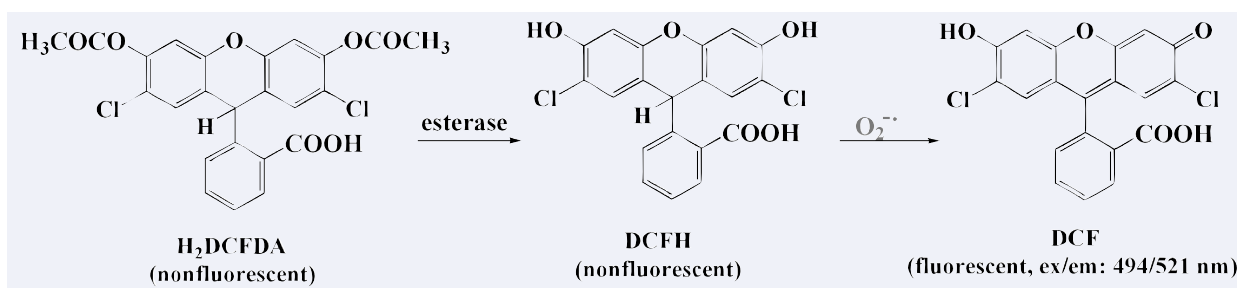
Fig. 6 The structures of H 2 DCFDA, DCFH and DCF; and the reaction pathway of superoxide detection. DCF has an absorption maximum at 494 nm and emission maximum of 521 nm.
