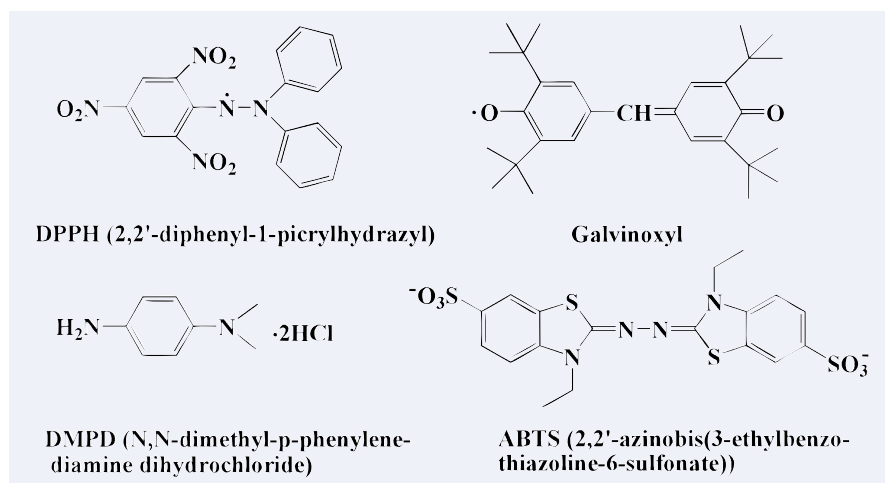
Fig. 9 Structures of DPPH, galvinoxyl, ABTS and DMPD.
