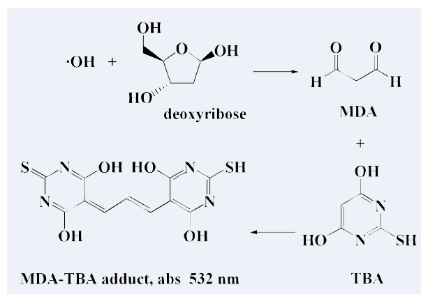
Fig. 8 Reaction pathway of TBARS assay of \cdot\text{OH} .
