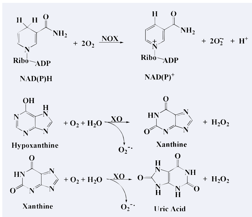
Fig. 10 Superoxide and hydroperoxide generation from NAD(P)H, oxidase (NOX) and XO.
