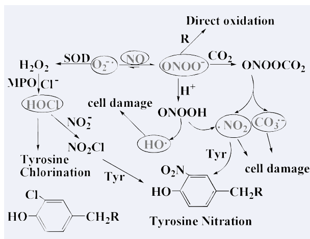
Fig. 13 Potential pathways of nitrotyrosine and chlorotyrosine formation. \text{ONOO}^- , peroxynitrite; \text{HOCl} , hypochlorous acid; \text{NO}_2\text{Cl} , nitryl chloride; \text{Cl}^- , chloride; \text{H}_2\text{O}_2 , hydrogen peroxide; \text{CO}_3^{\cdot-} , carbonate radical; \cdot\text{NO}_2 , nitrogen dioxide radical; \text{ONOOH} \text{NO}_2^- , peroxyntrous acid; \text{NO}_2\text{Cl} , nitryl chloride; MPO, myeloperoxidase; Tyr, tyrosine.
