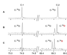
Figure 6. ^{13}\text{C} NMR spectra for C-1 and C-2 of 1-phenyl-1,2-ethanediol produced by NcsF2-catalyzed hydrolysis of: (A) racemic styrene oxide in \text{H}_2\text{O} ; (B) ( R )-styrene oxide in ^{18}\text{O} - \text{H}_2\text{O} (~80% final concentration); and (C) ( S )-styrene oxide in ^{18}\text{O} - \text{H}_2\text{O} (~60% final concentration).
