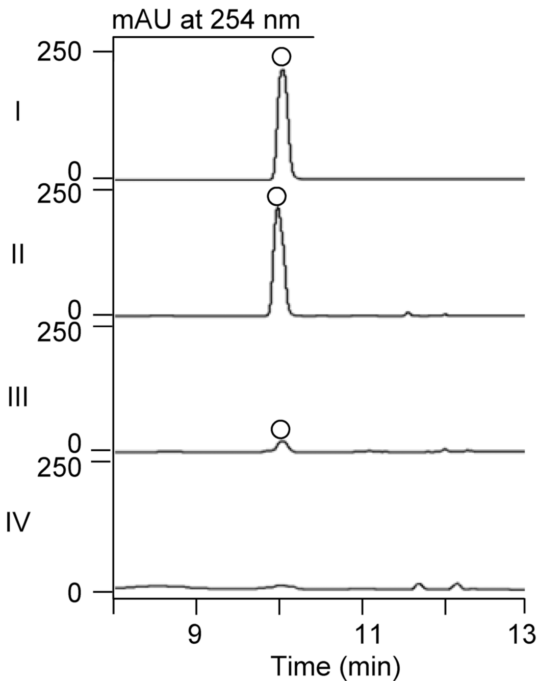
Figure 3. HPLC profiles for NcsF1- or NcsF2-catalyzed hydrolysis of racemic styrene oxide: (I) 1-phenyl-1,2-ethanediol standard (o); (II) with 50 \mu M NcsF2; (III) with 50 \mu M NcsF1; and (IV) with 50 \mu M NcsF2 (boiled) as a negative control.
