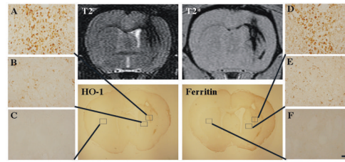
Figure 3. Heme oxygenase-1 (HO-1) and ferritin immunoreactivity in the brain 14 days after ICH. Scale bar (A-F) = 50 \mu m.
