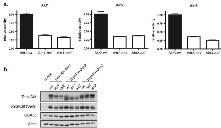
Fig. 2. (a) In vitro kinase activity of wt and analog sensitive ( as ) Akt kinases. (b) In vivo kinase activity of wt and as kinase activity. Myristoylated Akt was transfected into HEK293T cells and blotted for Akt substrates.
