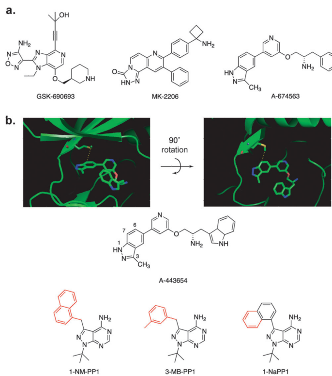
Fig. 1. (a) Structures of disclosed Akt inhibitors in clinical development. (b) Analog sensitive design strategy. Crystal structure of Akt2 with A443654 shows the native gatekeeper methionine and its proximity to the 7 position of indazole ring. Structures of PP1 derivatives commonly used to inhibit analog sensitive kinases.
