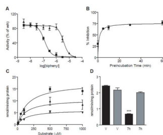
Figure 3. Characterization of NAAA inhibition by compound 7h in vitro. (A) Concentration-response curves for inhibition of NAAA by 7g ( meta -biphenyl derivative, closed triangles) and 7h ( para -biphenyl derivative, closed squares). (B) Preincubation time-course of 7h . (C) Michaelis-Menten analysis of 7h (vehicle – closed squares; 100 nM 7h : closed upright triangles; 200 nM 7h : closed inverted triangles). (D) Overnight dialysis of 7h (pre-dialysis: filled bars; post-dialysis: shaded bars). *** P < 0.001 vs vehicle-preincubation ( n = 3-5 ).
