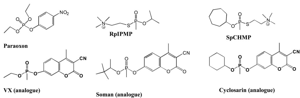
Figure 1. Structures of OP inhibitors used in this study.
