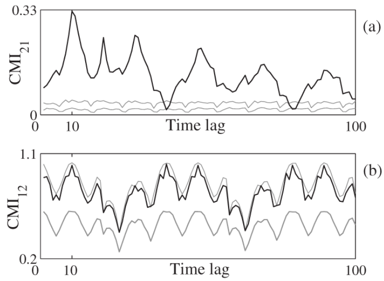
FIG. 5. (a) The CMI as a function of time lag (black) together with the surrogate ranges given by the surrogate mean \pm 1.96\sigma (gray) from 30 permutation surrogate realizations. For case (1), Fig. 4, the CMI is applied here with \Delta_{\tau \neq 1,2} according to Eq. (18).
