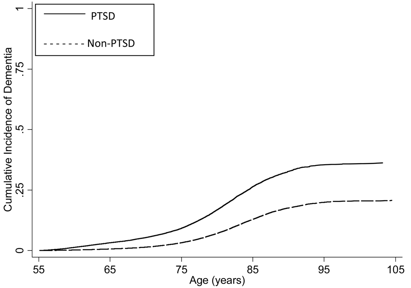
Figure. Cumulative incidence of dementia by age for all veterans
