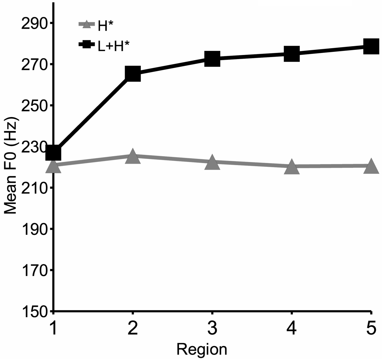
Figure 3. Mean F_0 contour of the stressed syllable for words in the H* and in the L+H* conditions in Experiment 2 materials.
