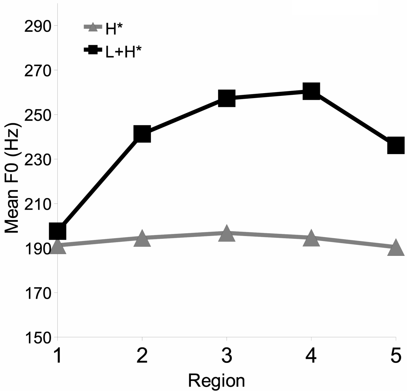
Figure 1. Mean F_0 contour of the stressed syllable for words in the H* and in the L+H* conditions in Experiment 1 materials. Note: The stressed syllable of each critical word was divided into five equal regions, and the mean F_0 was calculated across all items.
