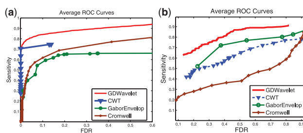
Fig. 5. ROC curves—simulated data with real noise and real data. Average ROC curves of four methods (Cromwell, CWT, GaborEnvelop and GDWavelet). (a) Obtained from 100 simulated MS signals in which real noise is used. There are 20–30 true peaks in this data. (b) Obtained from 60 MS signals (CAMDA, 2006). There are seven true peaks in this data.
